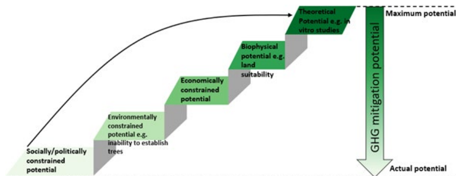
FIGURE 7 Relationship between theoretical maximum and actual GHG mitigation potential as influenced by social (barriers to adoption, animal welfare, social licence etc.), political (carbon price, red tape, emission mitigation legislation etc.), environmental (nutrient leaching, soil erosion, influence on biodiversity, ecosystems services etc.), economic (cost of implementation and relative return on investment etc.) and biophysical factors (climate, soil, geography, location etc). Social, political and environmental issues historically tend to be investigated last in studies of GHG emissions mitigation, whereas GHG emissions mitigation and productivity potentials are often evaluated first. Text adapted from Smith (2012)
