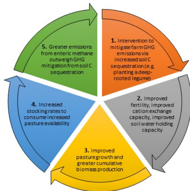
FIGURE 8 Example of a trade-off resulting from an intervention aimed at increasing soil carbon (e.g. through participation in an emissions trading scheme) that could result in higher net GHG emissions compared with business as usual. In the absence of external influence or constraints, landholders are likely to adapt grazing management to utilize any additional pasture or grassland production. This example illustrates the importance of assessing GHG emissions mitigation options holistically to manage unforeseen trade-offs, such as pollution swapping
