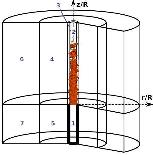
Figure 1: Sketch of seven block computational domain (not to scale).
