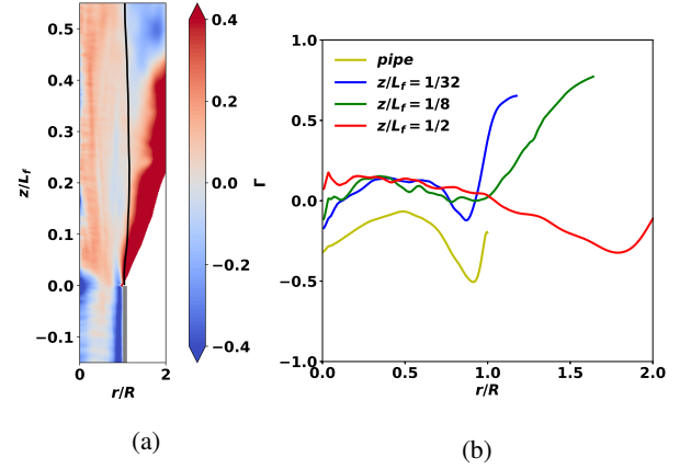
Figure 4: (a) Spanwise average of \Gamma with black line denoting the flame front based on iso-contour of \tilde{Y}_R = 0.134 (b) profiles of \Gamma at four streamwise locations. Regions with turbulence intensity < 1\% are filtered.
