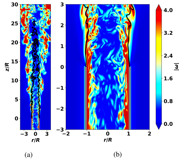
Figure 2: Instantaneous contours of the vorticity magnitude and Y_R = 0.134 iso-surface (black line) (a) with view of entire flame and surrounding field, and (b) in the region of the pipe exit.
