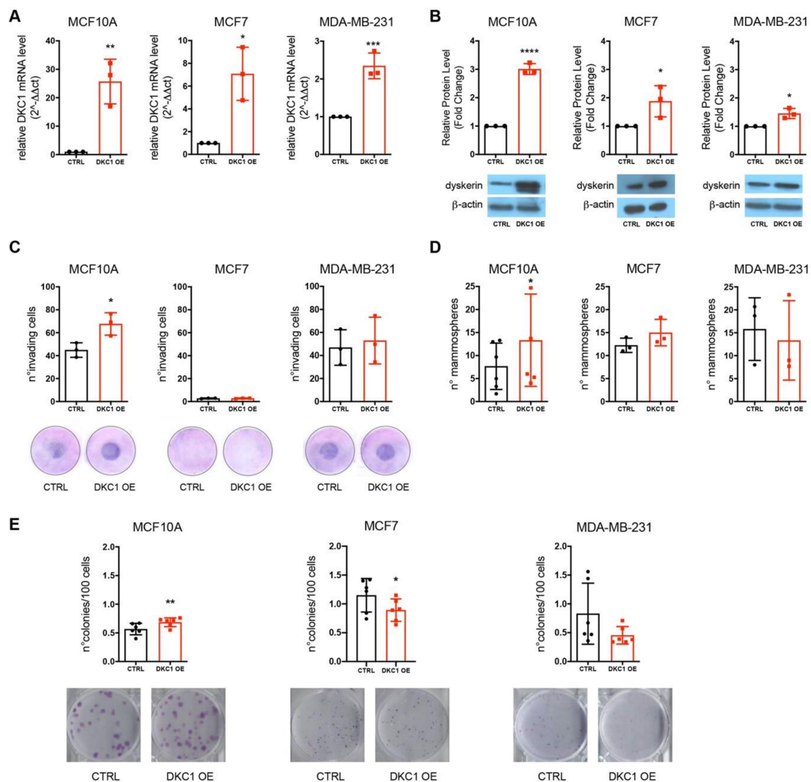
Figure 2. DKC1 overexpression confers a more aggressive cellular phenotype to immortalized mammary gland epithelial cells. (A) DKC1 mRNA expression evaluated by RT-qPCR. Results are shown as fold change respect to CTRL, set to 1 for all the three cell lines. (B) Dyskerin expression by Western blot analysis. Results are shown as fold change respect to CTRL, set to 1 for all the three cell lines. (C) Invasive potential assay through blind well assay chambers. For each filter sample five random fields were counted. Graphs show the total number of cells counted in each filter. (D) Stemness potential assay through mammospheres formation. Due to the intrinsic subjective nature of the experiment, we repeated it six times for MCF10A. (E) Clonogenic potential assay. At least n = 3 biological and technical replicates were performed for each experiment. All data were analyzed by paired Student's T -test. * p < 0.05 ; ** p < 0.01 ; *** p < 0.001 , **** p < 0.0001 . The error bars indicate the SD.
