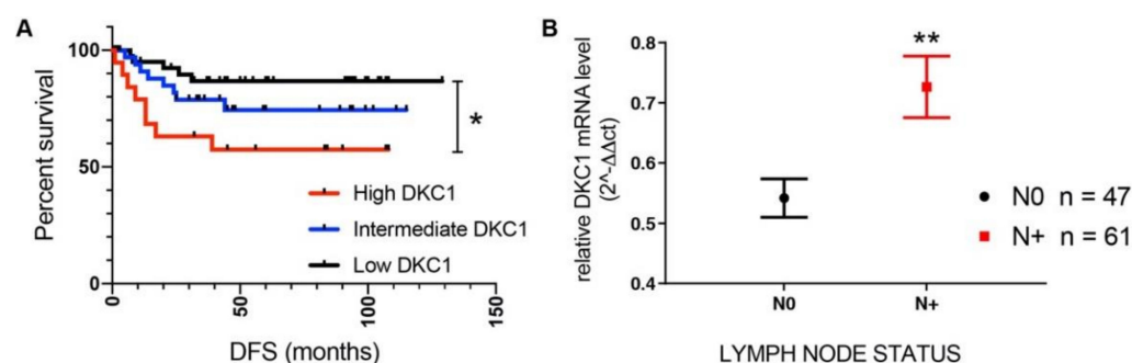
Figure 1. DKC1 overexpression is related to patients' worse prognosis. (A) Disease free survival (DFS) of patients who had undergone surgery for primary breast carcinoma according to cancer cells DKC1 mRNA expression. Low DKC1 n = 54 mean expression value 0.39 \pm 0.08 a.u.; Intermediate DKC1 n = 48 mean expression value 0.68 \pm 0.10 a.u.; High DKC1 n = 22 mean expression value 1.25 \pm 0.08 a.u. Data were analyzed by Mantel–Cox and Gehan–Breslow–Wilcoxon tests. * p < 0.05 . (B) DKC1 mRNA expression and lymph node status in primary breast carcinomas. Data were analyzed by Mann–Whitney–test ** p < 0.01 . The error bars indicate the SD.
