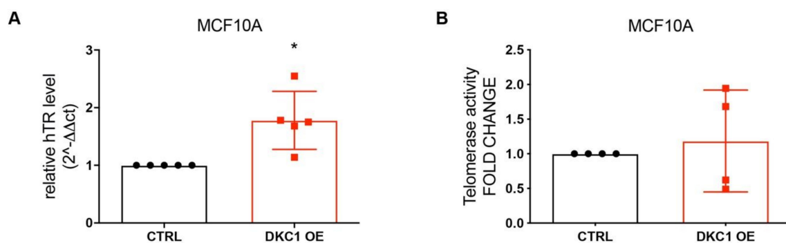
Figure 3. DKC1 overexpression leads to an increase in human telomerase RNA (hTR) levels without influencing telomerase complex activity. (A) Evaluation of hTR levels in Real-Time PCR. Data were analyzed by paired Student's T -test: * p < 0.05. The error bars indicate the SD. (B) Telomerase activity assay. Statistical analyses have been conducted following protocol instructions. At least n = 3 biological and technical replicates were performed for each experiment.
