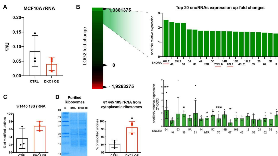
Figure 4. DKC1 overexpression did not influenced global rRNA pseudouridylation, but induced a remodeling in snoRNAs expression levels and a site-specific pseudouridylation increase in U1445 on 18S rRNA. (A) HPLC analysis of ribosomal RNA (rRNA) extracted from highly purified ribosomes. Results are shown as \Psi /U ratio. (B Left) Heat map of all H/ACA box small nucleolar RNA (snoRNAs) ordered by fold change (DKC1 OE/CTRL) LOG2. Green values are for more expressed snoRNAs, red values for less expressed. (B Right) Focus on top 20 up-regulated snoRNAs in MCF10A Dyskerin overexpressing cells from Arraystar expression array analyses (up). snoRNAs expression validated by RT-qPCR (down). Data were analyzed by paired Student's T -test * p < 0.05 ; ** p < 0.01 ; *** p < 0.001 . The error bars indicate the SD. (C) LC-MS analyses of \Psi 1445 on 18S rRNA and (D right) on RNA from cytoplasmic ribosomes. Results are shown as percentage of modified uridines and were calculated from the peak area. Data were analyzed by unpaired Student's T -test * p < 0.05 . The error bars indicate the SD. (D left) Coomassie stain of a PAGE of proteins from the purified ribosomes. Note that following the purification procedure only bands of sizes corresponding to ribosomal proteins were detected. At least n = 3 biological and technical replicates were performed for each experiment.
