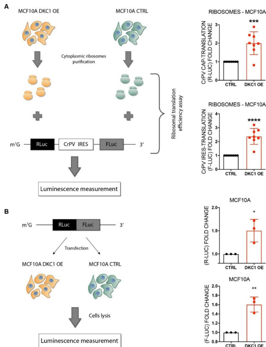
Figure 5. DKC1 overexpression provides ribosomes with increased translational efficiency in MCF10A cells. (A) mRNA translation efficiency assay conducted on highly purified ribosomes extracted from MCF10A DKC1 overexpressing cells and control cells. (B) mRNA translation efficiency assay on MCF10A DKC1 overexpressing and control cells. At least n = 3 biological replicates were performed, testing all sample in duplicate. Data were analyzed by unpaired or paired Student's T -test as appropriate. * p < 0.05 ; ** p < 0.01 ; *** p < 0.001 ; **** p < 0.0001 . The error bars indicate the SD.
