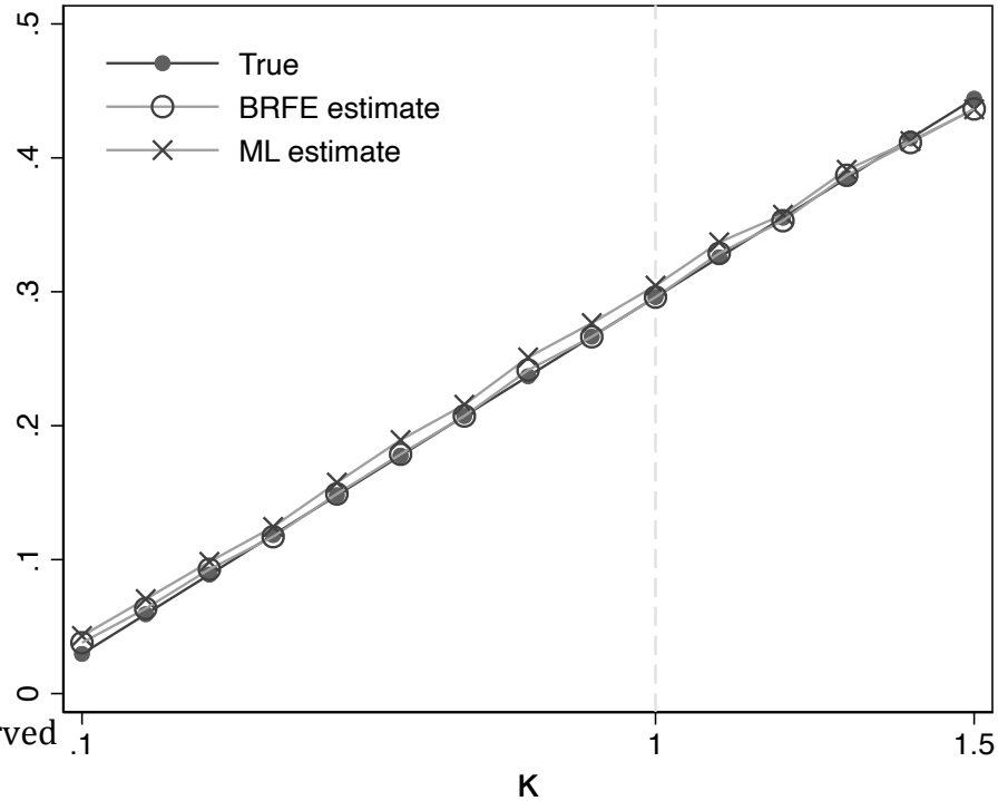
STANDARD DEVIATION, T=8
