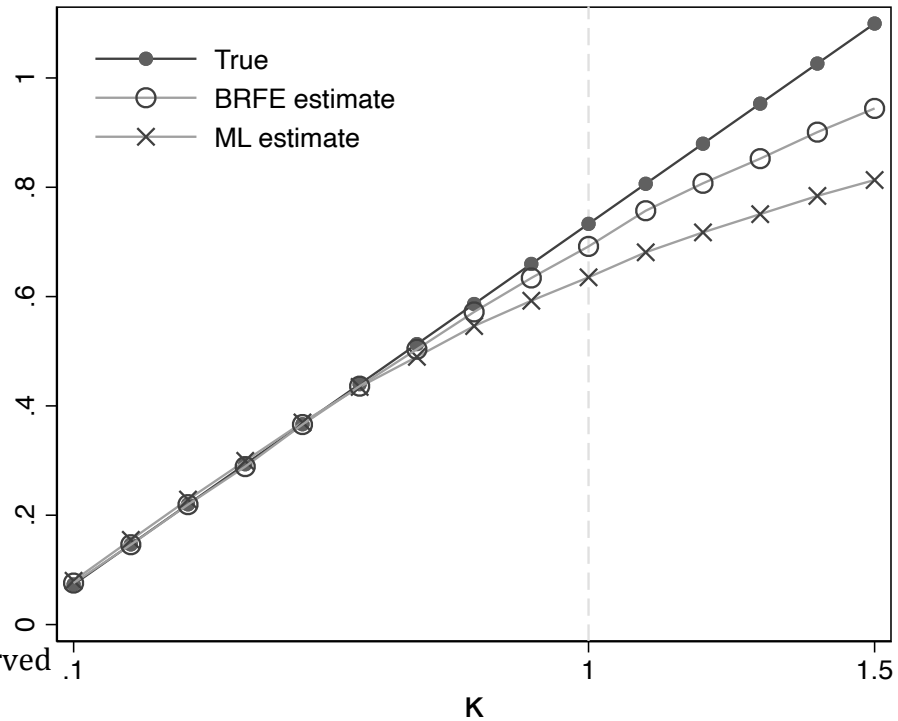
STANDARD DEVIATION, T=8
