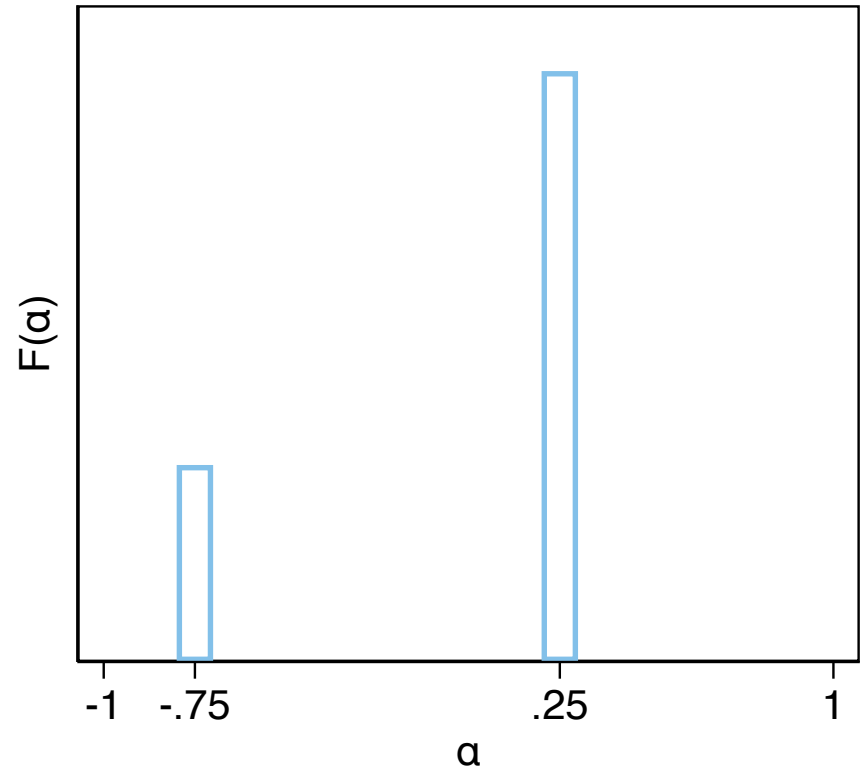
\alpha \sim \text{bernoulli}
