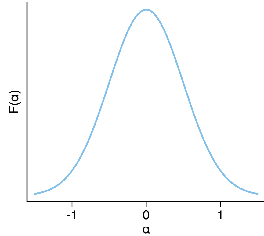
\alpha \sim \text{normal}
