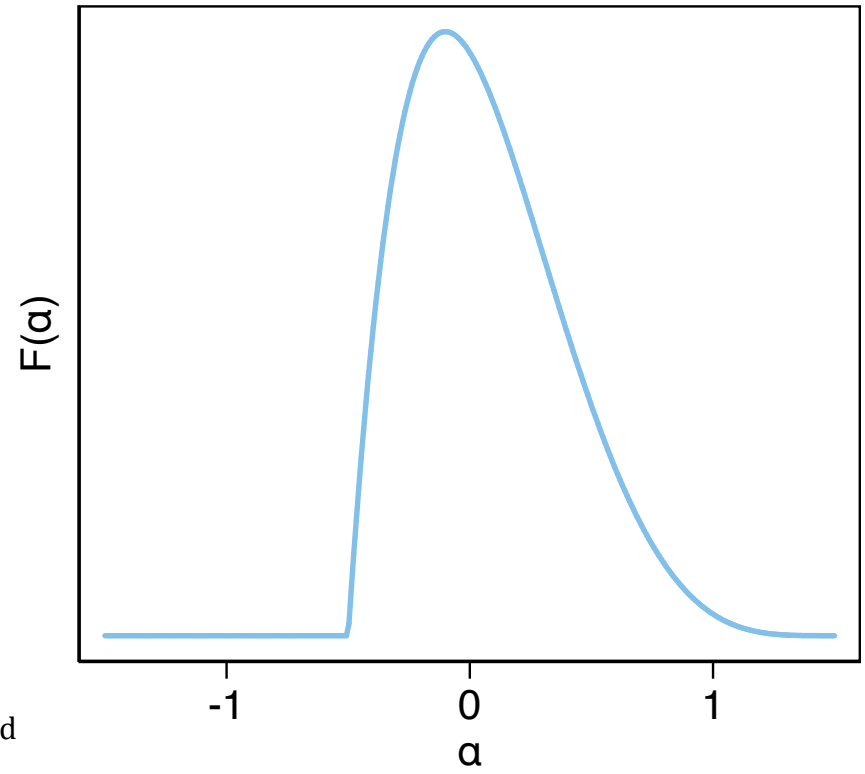
\alpha \sim \text{beta}
