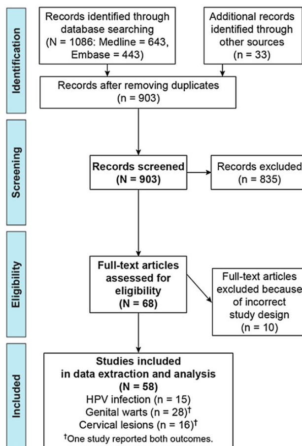
Figure 1. PRISMA (Preferred Reporting Items for Systematic Reviews and Meta-Analyses) diagram. Details of literature search and extraction for our systematic review. Abbreviation: HPV, human papillomavirus.
