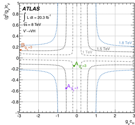
Fig. 4 Observed 95% CL exclusion contours in the HVT parameter space \{(g^2/g_V)c_F, g_V c_H\} for resonances of mass 1 TeV, 1.5 TeV and 1.8 TeV. The areas outside the curves are excluded. Also shown are the benchmark model parameters A(g_V = 1) , A(g_V = 3) and B(g_V = 3)
