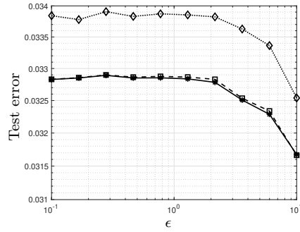
Fig. 2 Performance of the linear regression for the Loan dataset trained on the locally-differential private dataset tested on the original probability distribution using (9) (solid), without any regularization (dashed), and using \ell_2 -norm regularization (dotted).
