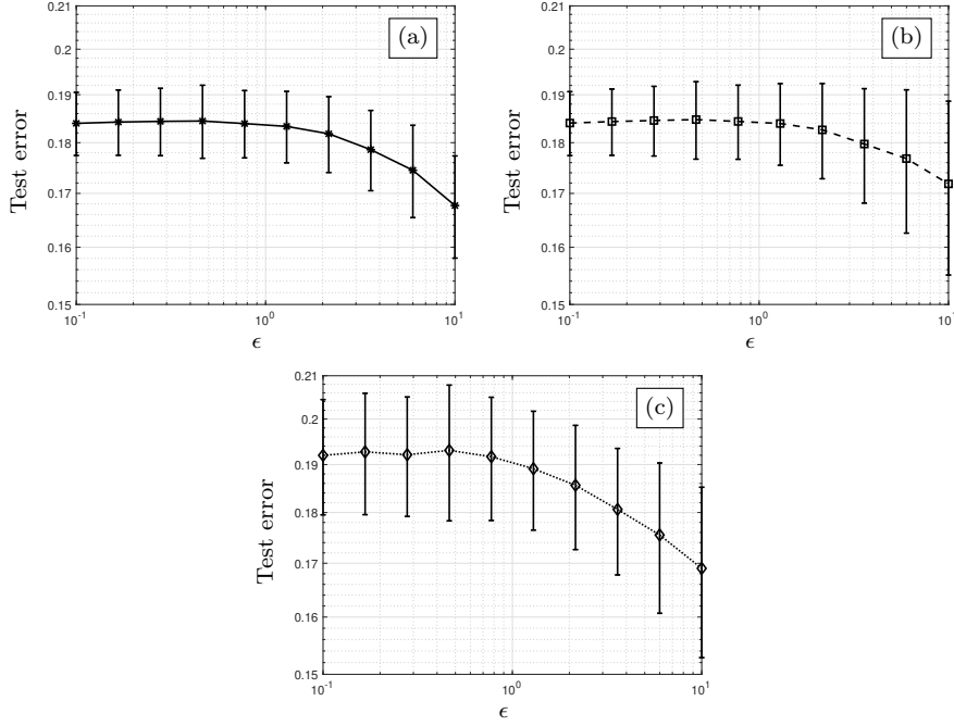
Fig. 3 Performance of the linear regression for the Adult dataset trained on the locally-differential private dataset tested on the original probability distribution using (9) [a], without any regularization [b], and using \ell_2 -norm regularization [c].
