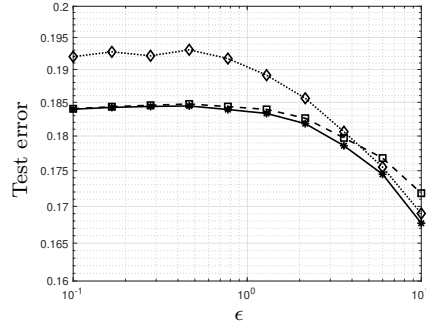
Fig. 4 Performance of the linear regression for the Adult dataset trained on the locally-differential private dataset tested on the original probability distribution using (9) (solid), without any regularization (dashed), and using \ell_2 -norm regularization (dotted).
