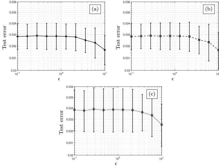
Fig. 1 Performance of the linear regression for the Loan dataset trained on the locally-differential private dataset tested on the original probability distribution using (9) [a], without any regularization [b], and using \ell_2 -norm regularization [c].
