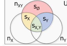
Fig. 2: Neighbourhoods of a query along the individual distance variables, i.e., X and Y as well as their joint distance variable XY .
