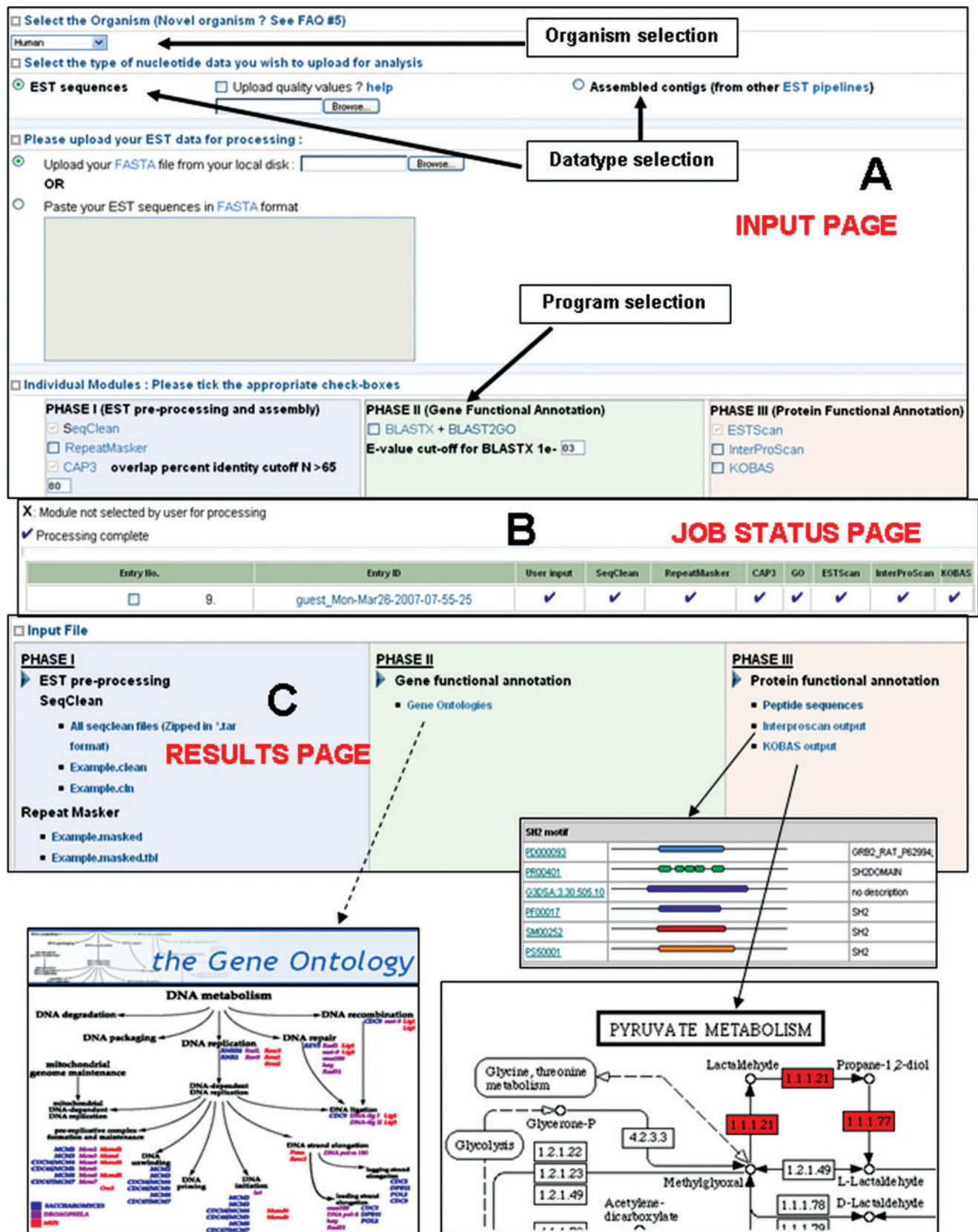
Figure 1. ESTExplorer input and analysis output pages. (A) EST or contig submission with optional parameters for organism and program selection, (B) Status page to monitor the progress of different programs and (C) Result download page from where processed data can be downloaded and annotation links accessed. Screenshots of the results showing Gene Ontologies (accessed via a link for each EST/contig), InterProScan and KEGG pathway mapping obtained from processed EST data are shown.
