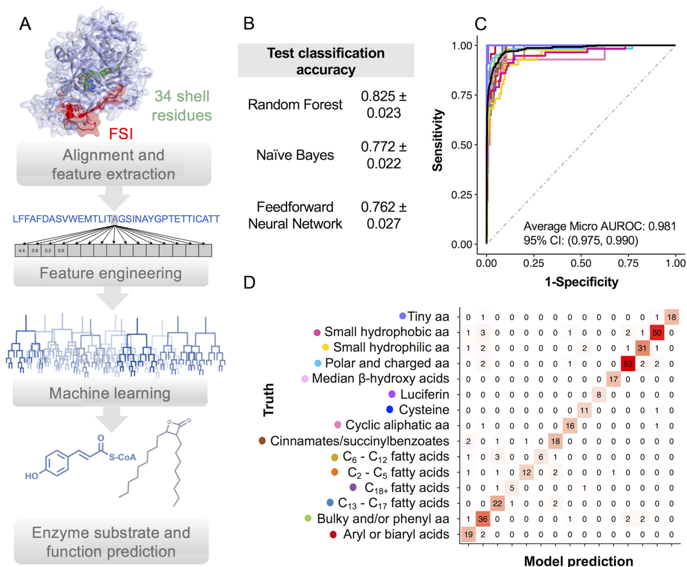
Figure 1. Machine learning to predict substrate and function of adenylate-forming enzymes from protein sequences. A, the machine learning workflow includes extracting 34 active site residues (green) and FAAL-specific loop (red) residues and encoding them as a vector of physiochemical properties. Separate classifiers are trained to predict substrate specificity and enzyme function. B, hold-out test set accuracy scores for three different classification methods evaluated in this study. C, AUROC for substrate specificity predictions. Colors correspond to different substrates and macro (gray) and micro (black) AUROC averages. Red, aryl/biaryl acids; green, bulky/phenyl aa; blue, C 13 –C 17 fatty acids; purple, C 18 + fatty acids; orange, C 2 –C 5 acids; tan, C 6 –C 12 fatty acids; brown, succinylbenzoic acids; hot pink, cyclic aliphatic aa; dark blue, cysteine; fuchsia, luciferin; light pink, β-hydroxy acids; turquoise, polar and charged aa; goldenrod, small hydrophilic aa; deep pink, small hydrophobic aa; lavender, tiny aa. D, confusion matrix of predicted versus truth for ANL substrate specificity on hold-out test set. Predictions for functional class are presented in Fig. S2.
