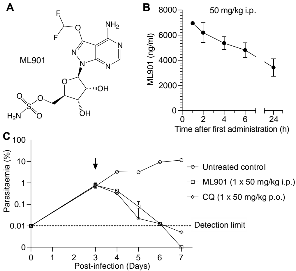
Figure 2. ML901 exhibits potent activity against P. falciparum in vivo. (A) Structure of pyrazolopyrimidine ribose sulfamate, ML901. (B) Pharmacokinetics profile (in blood) over the first day for SCID mice engrafted with human RBCs infected with P. falciparum following treatment with ML901 at 50 mg/kg i.p. (C) Therapeutic efficacy of ML901 in the SCID mouse P. falciparum model, dosed with ML901 at 50 mg/kg i.p. in comparison with gold standard antimalarial, chloroquine, dosed at 50 mg/kg p.o..
