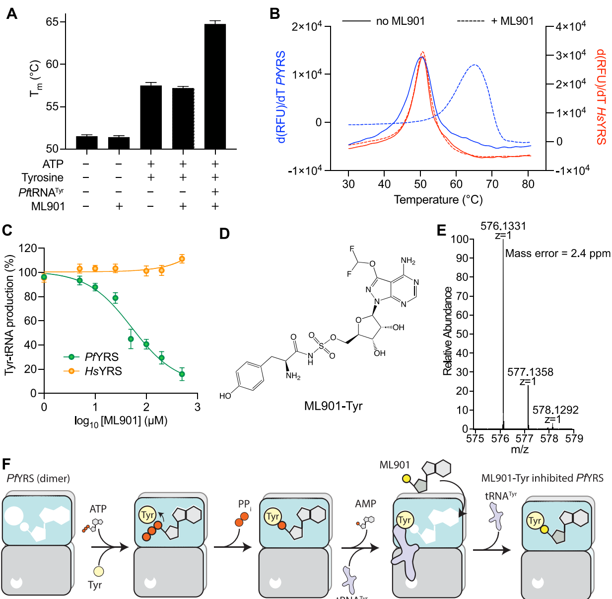
Figure 4. ML901 inhibits PfYRS by a reaction-hijacking mechanism. (A) The apparent melting temperature ( T_m ) of PfYRS after incubation at 37°C for 3 h with the indicated reactants: ML901 (50 \mu M), ATP (50 \mu M), tyrosine (100 \mu M), PftRNA Tyr (4 \mu M). Data represent the average of three independent assays and error bars correspond to SD. (B) First derivatives of melting curves for PfYRS and HsYRS with or without pre-incubation with ML901 (50 \mu M), ATP (50 \mu M), tyrosine (100 \mu M) and PftRNA Tyr (4 \mu M). Data is representative of three independent assays. (C) Effects of increasing concentrations of ML901 on tyrosine acylation of the cognate tRNA Tyr by PfYRS and HsYRS with YRS (0.25 \mu M), ATP (10 \mu M), tyrosine (100 – 200 \mu M), cognate tRNA Tyr (24 \mu M) and pyrophosphatase (1 unit/mL), at 37°C for 1 h. IC_{50} ( PfYRS ) = 53 \mu M; IC_{50} ( HsYRS ) > 500 \mu M. Data represent the average of 8 independent assays and error bars correspond to SEM. (D) Structure of ML901-Tyr. (E) PfYRS was incubated with ML901 (50 \mu M), ATP (10 \mu M), tyrosine (20 \mu M) and PftRNA Tyr (8 \mu M). Following urea denaturation and TFA precipitation, the supernatant was subjected to LCMS analysis, revealing the expected protonated ML901-Tyr ion. The profile is typical of data from three independent experiments. (F) Schematic of reaction-hijacking mechanism.
