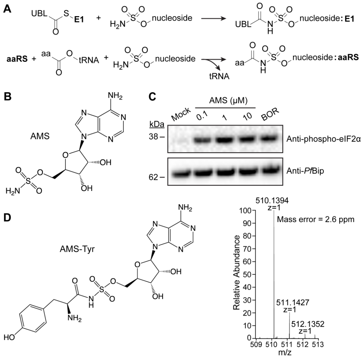
Figure 1. AMS-treated infected RBCs reveals aaRSs as potential targets. (A) E1 enzymes can catalyze attack of the sulfamate nitrogen on the carbonyl carbon of the thioester bond between the UBL and the E1 to form a UBL conjugate. aaRSs could catalyze nucleoside sulfamate attack on activated amino acids to form an amino acid adduct. (B) Structure of 5'-adenylate sulfamate. (C) Trophozoite stage parasites were incubated with DMSO (Mock), different concentrations of AMS, or, borrelidin (BOR; a threonyl-tRNA synthetase inhibitor). Western blots of lysates were probed for phosphorylated-eIF2 \alpha with PfBiP as a loading control. The blot is typical of data from three independent experiments. (D) P. falciparum -infected RBCs were treated with 10 \mu M AMS for 3 h. Extracts were subjected to LCMS analysis identifying the Tyr-AMS conjugate. The profile is typical of data from three independent experiments.
