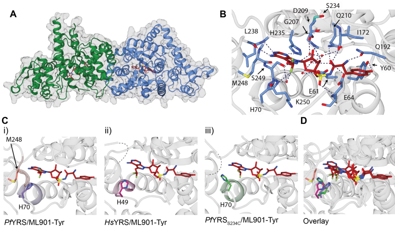
Figure 5. Structural analysis of YRSs reveals the determinants of potency and specificity. (A) The structure of the dimeric PfYRS /ML901-Tyr complex showing chain A (green), chain B (blue), and bound ML901-Tyr (red stick representation). (B) Inhibitor/active site interactions for the B chain. (C) (i) The PfYRS chain B active site highlighting the “HIGH” ( 70 HIAQ 73 ; light purple) and “KMSKS” ( 247 KMSKS 251 ; light brown) motifs with bound ML901-Tyr (colored by atom type). M248 and H70 are positioned to interact. (ii) Active site of HsYRS with bound ML901-Tyr highlighting the “HIGH” motif ( 49 HVAY 52 ; light pink). (iii) Active site of PfYRS S234C with bound ML901-Tyr highlighting the “HIGH” ( 70 HIAQ 73 ; light green). Unmodelled loops are shown in Cii and Ciii as dashed lines. (D) Overlay of PfYRS (B chain), HsYRS , and PfYRS S234C showing the different configurations adopted by His70/His49. PfYRS His70, purple; HsYRS His49, pink; PfYRS S234C His70, green.
