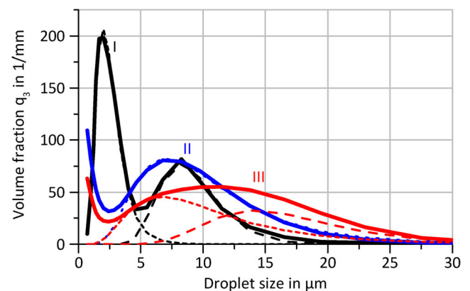
Fig. 9 Measured droplet size distributions (volume fraction q_3 , averages of 3x15s measurements) for three chosen combinations of flow rate and power (Fig. 8); logarithmic normal distribution functions fitted to individual peaks indicated by dashed lines (the addition of individual fitted functions results in almost ideal reproduction of the measured curve)
