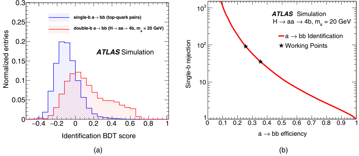
FIG. 2. (a) Identification BDT score distributions for signal and background a \rightarrow b\bar{b} candidates and (b) signal efficiency as a function of the inverse of the t\bar{t} background efficiency (rejection). For the signal H \rightarrow aa \rightarrow (b\bar{b})(b\bar{b}) sample with m_a = 20 GeV, both b quarks are required to lie within the reconstructed candidate, while for the background t\bar{t} sample the reconstructed candidate contains a single b quark. In panel (b), the left and right stars indicate the tight and the loose WPs, respectively, which are used to define, as described in the text, the HPC and LPC.
