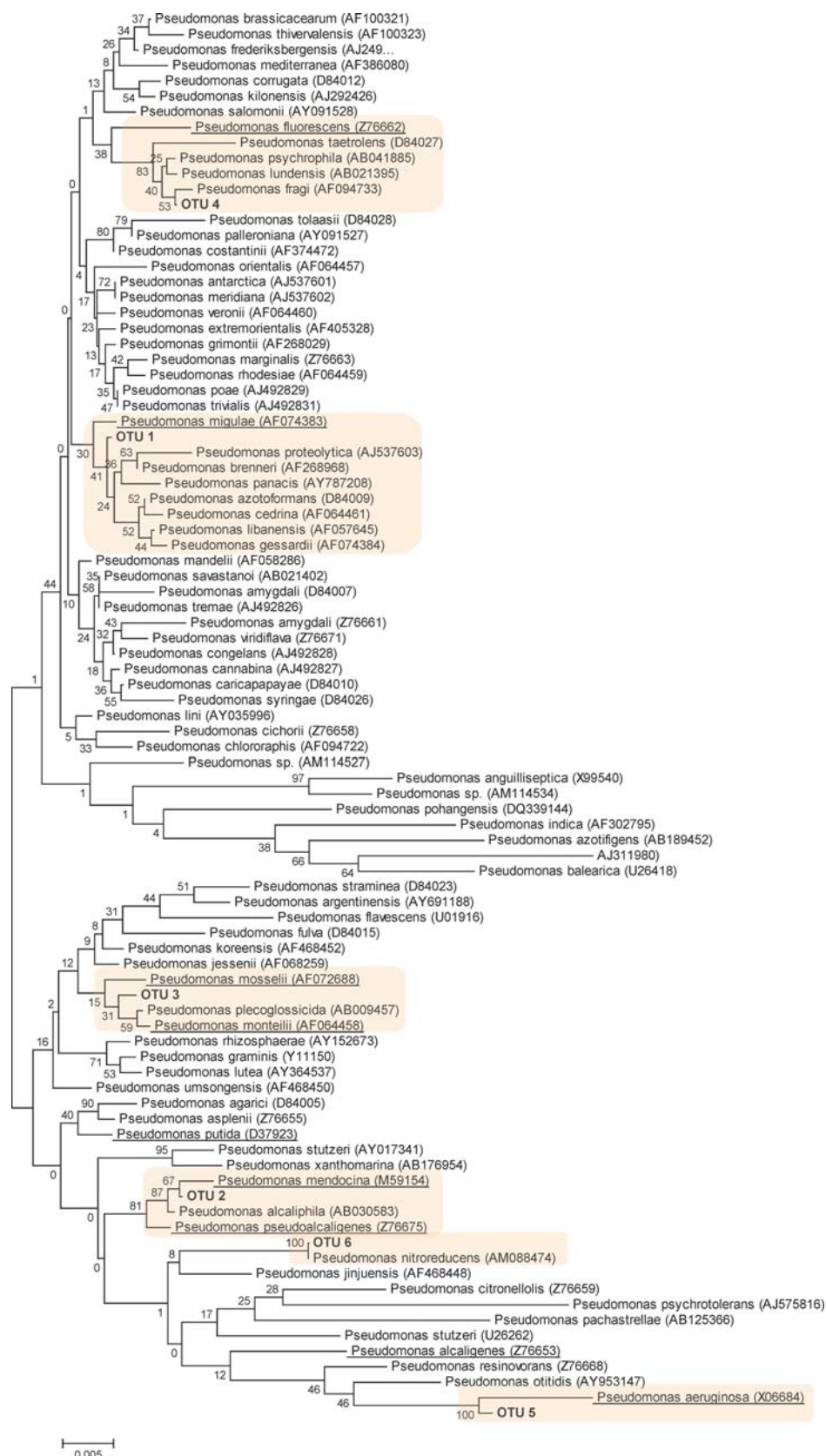
Figure 2. Phylogenetic tree generated from Pseudomonas type strains and consensus sequences from OTUs (OTU1-6) at sequence similarity threshold of 97%. Bootstrap values are base on 500 replications. The scale bar represents the nucleotide substitution per site. Underlined reference sequences are known human pathogenic strains. Shaded box are considered as closely related species within each OTU group. doi:10.1371/journal.pone.0003578.g002
