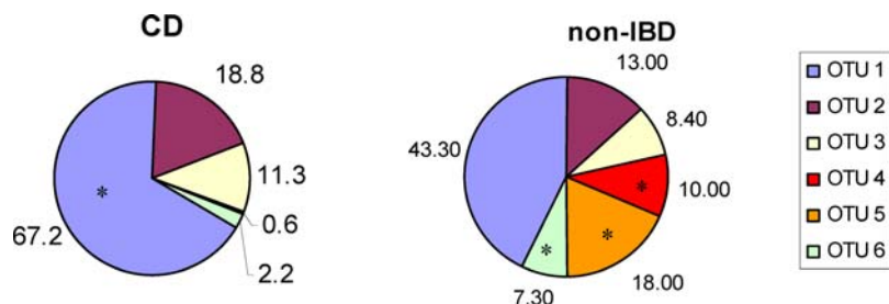
Figure 1. Diversity analysis of Pseudomonas 16S ribosomal sequences obtained from Crohn's disease patients and non-inflammatory bowel disease control patients. Five hundred and eighty one sequences from the Crohn's disease (CD) and non-inflammatory bowel disease (non-IBD) patient libraries were grouped into operational taxonomic units (OTU) using a sequence similarity threshold of 97%. The fraction of sequences in each OTU and patient group were calculated and presented. * Significant more sequences in these OTUs compared to the other patient group ( p < 0.01 , Fisher exact test). doi:10.1371/journal.pone.0003578.g001
