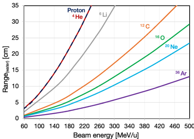
Figure 4: Approximated range of proton and helium, lithium, carbon, oxygen, neon and argon ions in water as dependent on beam energy.
