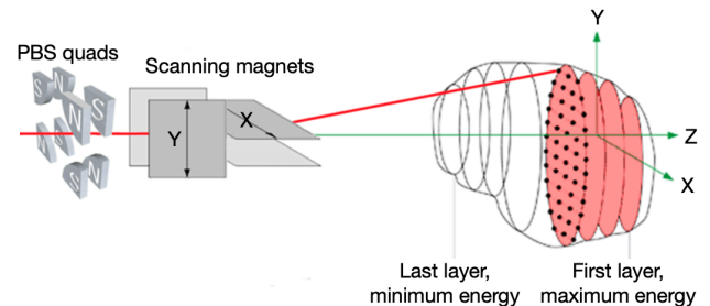
Figure 1: PBS delivery. Scanning magnets deflect the beam which traces across a target volume, superimposed in multiple layers to deliver a conformal 3D dose distribution. Adapted from [6].
