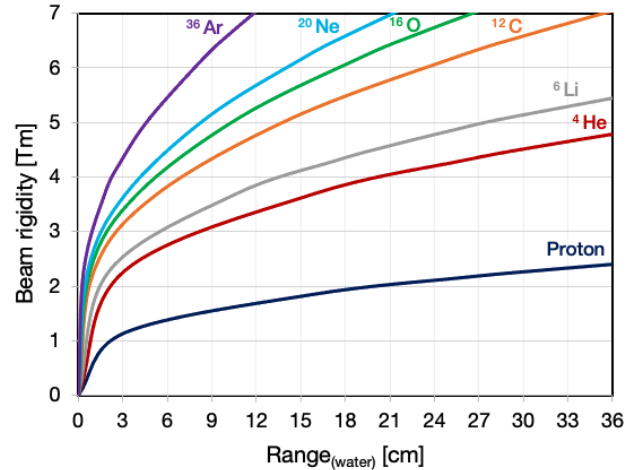
Figure 5: Beam rigidity of different ion beams across therapeutic depths.
