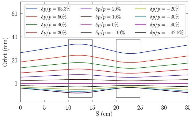
Figure 3: Varying beam energies as transported through a single doublet cell of the FFA bend.
