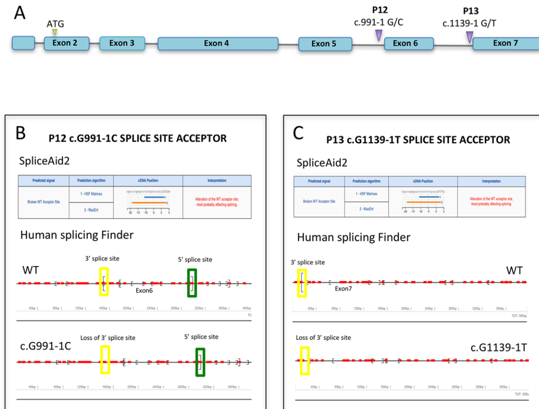
FIGURE 2 Splice site mutations identified in 46,XY individuals. A: A schematic representation of NR5A1 , showing the six coding exons and the position of the two splice site acceptor mutations identified. B and C: Human Splicing Finder (Desmet et al., 2009) and SpliceAid 2 (Piva et al., 2012) were used to analyze the consequences of the two splice site acceptor mutations. Both of which suggest that wild-type splicing would be affected
