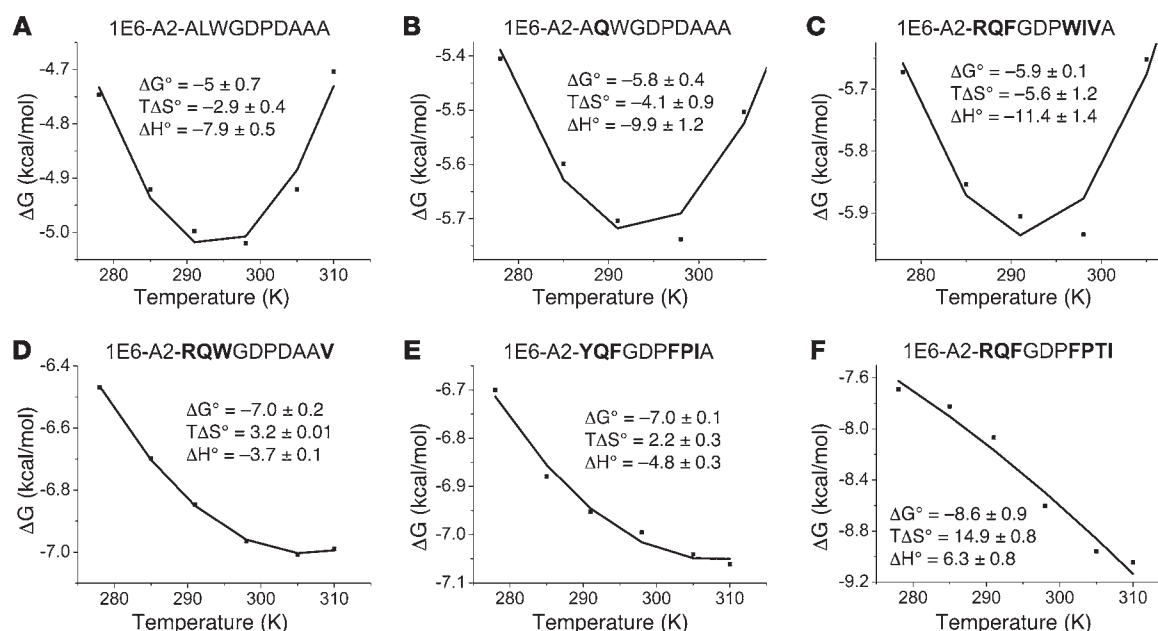
Figure 8. Thermodynamic analysis of the 1E6 TCR with A2-ALWGPDPAAAA and the APLs. Eight serial dilutions of the 1E6 TCR were injected, in duplicate, over each immobilized APL and A2-ALW at 5°C, 13°C, 18°C, 25°C, 30°C, and 37°C. The equilibrium binding constant ( K_D ) values were calculated using a nonlinear curve fit ( y = [P_x]/[P_x + X] ), and thermodynamic parameters were calculated according to the Gibbs-Helmholtz equation ( \Delta G^\circ = \Delta H - T\Delta S^\circ ). The binding free energies, \Delta G^\circ ( \Delta G^\circ = RT \ln K_D ), were plotted against temperature (K) using nonlinear regression to fit the 3-parameters van't Hoff equation ( RT \ln K_D = \Delta H^\circ - T\Delta S^\circ + \Delta C_p [T - T_0] - T\Delta C_p \ln [T/T_0] with T_0 = 298 K). (A) 1E6-A2-ALWGPDPAAAA; (B) 1E6-A2-AQWGPDPAAAA; (C) 1E6-A2-RQFGDPWIVA; (D) 1E6-A2-RQWGPDPAAV; (E) 1E6-A2-YQFGDPFPTA; and (F) 1E6-A2-RQFGDPFPTI.
