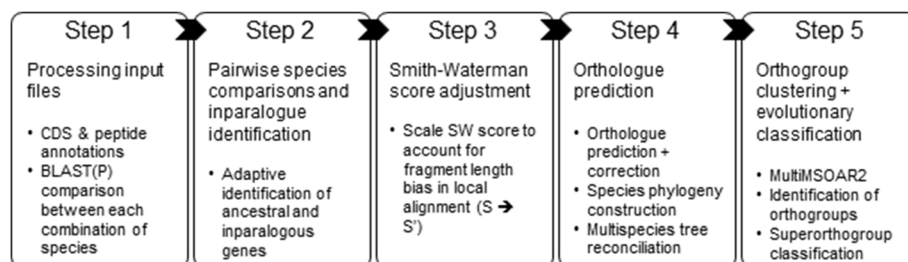
Fig. 1 Process flow diagram for the Orthonome pipeline. The five-step pipeline combines the power of heuristic and greedy algorithms to improve the accuracy and recall from both well annotated and draft genomes
