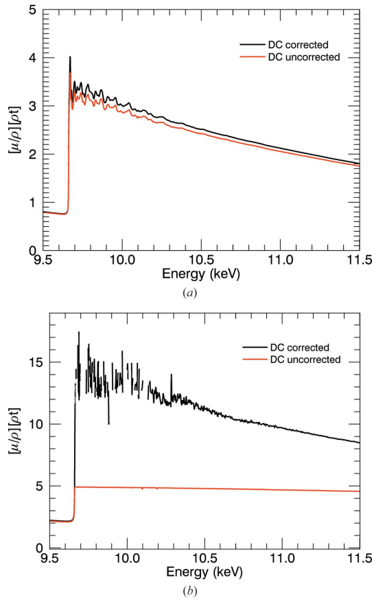
Figure 5 The effect of correcting for dark current in the 10 K data for the (a) 10 \mu\text{m} foil and (b) 50 \mu\text{m} foil. At 10 \mu\text{m} , the largest displacement is near the absorption edge. The largest glitch in the uncorrected data, near to 10.1 keV, disappears after correction for dark current. For 50 \mu\text{m} , correcting for the dark current reveals some consistency in the spectra at high k . It is quite important to monitor the dark current through a spectral data collection.
