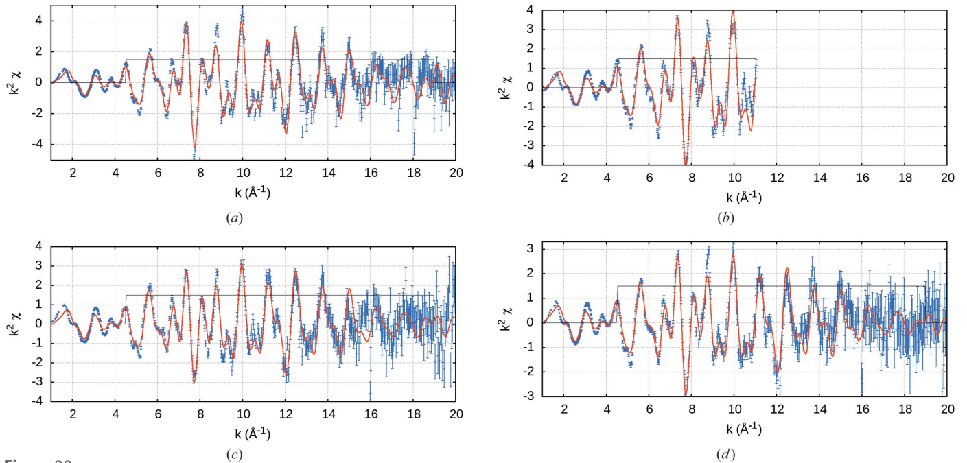
Figure 22 Fluorescence XAFS spectra in k^2\chi versus k and theoretical fits at (a) 10 K, (b) 50 K, (c) 100 K and (d) 150 K. The fit follows the data very closely, even below the fitting window.
