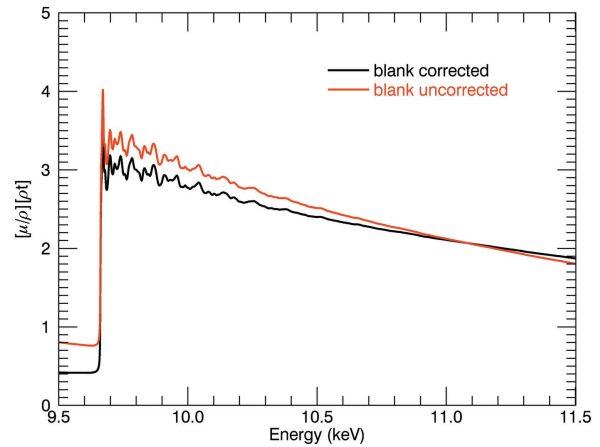
Figure 6 Change in spectra due to blank correction at 10 K for the 10 \mu\text{m} foil. Red: corrected for dark current; black: corrected for blank and dark current, with a reduction of 52.9% pre-edge, and significant change to the slope.
