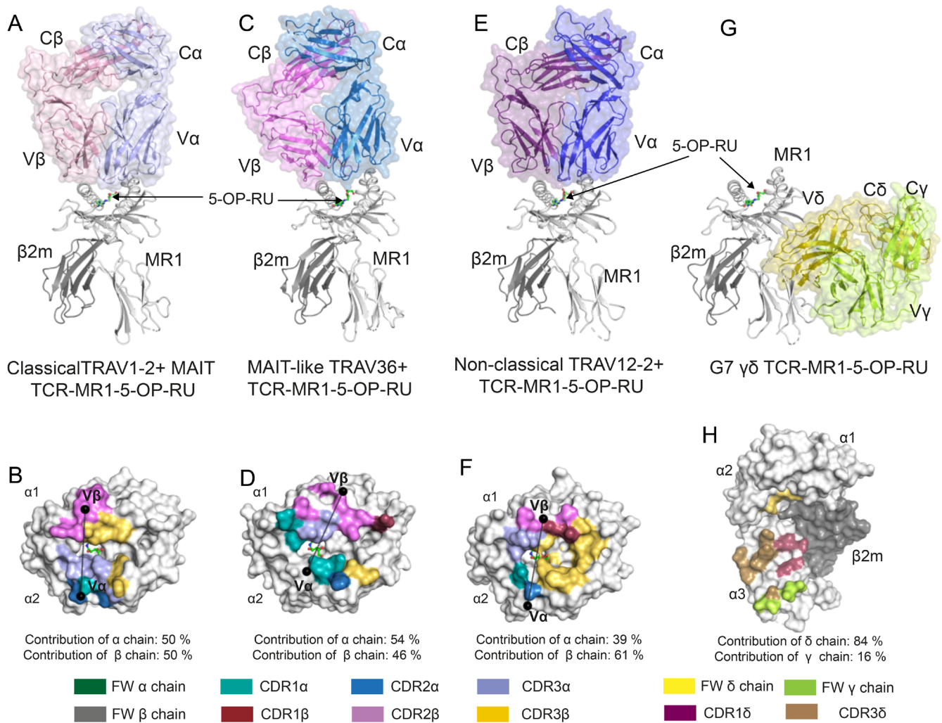
FIGURE 5 | Crystal structures of the ternary complexes of (A, B) A-F7 TCR-MR1-5-OP-RU (PDB; 4NQC), (C, D) TRAV36 + TCR-MR1-5-OP-RU (PDB; 5D7L), (E, F) non-classical TRAV12-2 + TCR-MR1-5-OP-RU (PDB; 6XQP), and (G, H) G7 \gamma\delta TCR-MR1-5-OP-RU (PDB; 6MWR). Top panels (A, C, E, G) show ribbon diagrams of the ternary complexes. The MR1 and \beta 2-microglobulin molecules are colored white and gray, respectively, and 5-OP-RU is presented as green sticks. A-F7 TCR \alpha , light blue; A-F7 TCR \beta , pink; MAV36 TCR \alpha , sky blue; MAV36 TCR \beta , violet; TRAV12-2 TCR \alpha , slate; TRAV12-2 TCR \beta , violet-purple; TCR \gamma , lemon; G7 TCR \delta , yellow orange. The lower panels (B, D, F, H) illustrate the TCR footprints on the molecular surface of MR1-5-OP-RU. The centers of mass of the TCR variable domains are shown as black spheres. The atomic footprints of CDR loops are colored as follows: CDR1 \alpha , teal; CDR2 \alpha , sky blue; CDR3 \alpha , light blue; Frameworks of \alpha -chain, dark green; CDR1 \beta , maroon; CDR2 \beta , violet; CDR3 \beta , yellow orange; Frameworks of \beta -chain, dark gray; Frameworks of \delta chain, yellow orange; Frameworks of \gamma chain, Lemon; CDR1 \delta , raspberry; CDR3 \delta , yellow olive.
