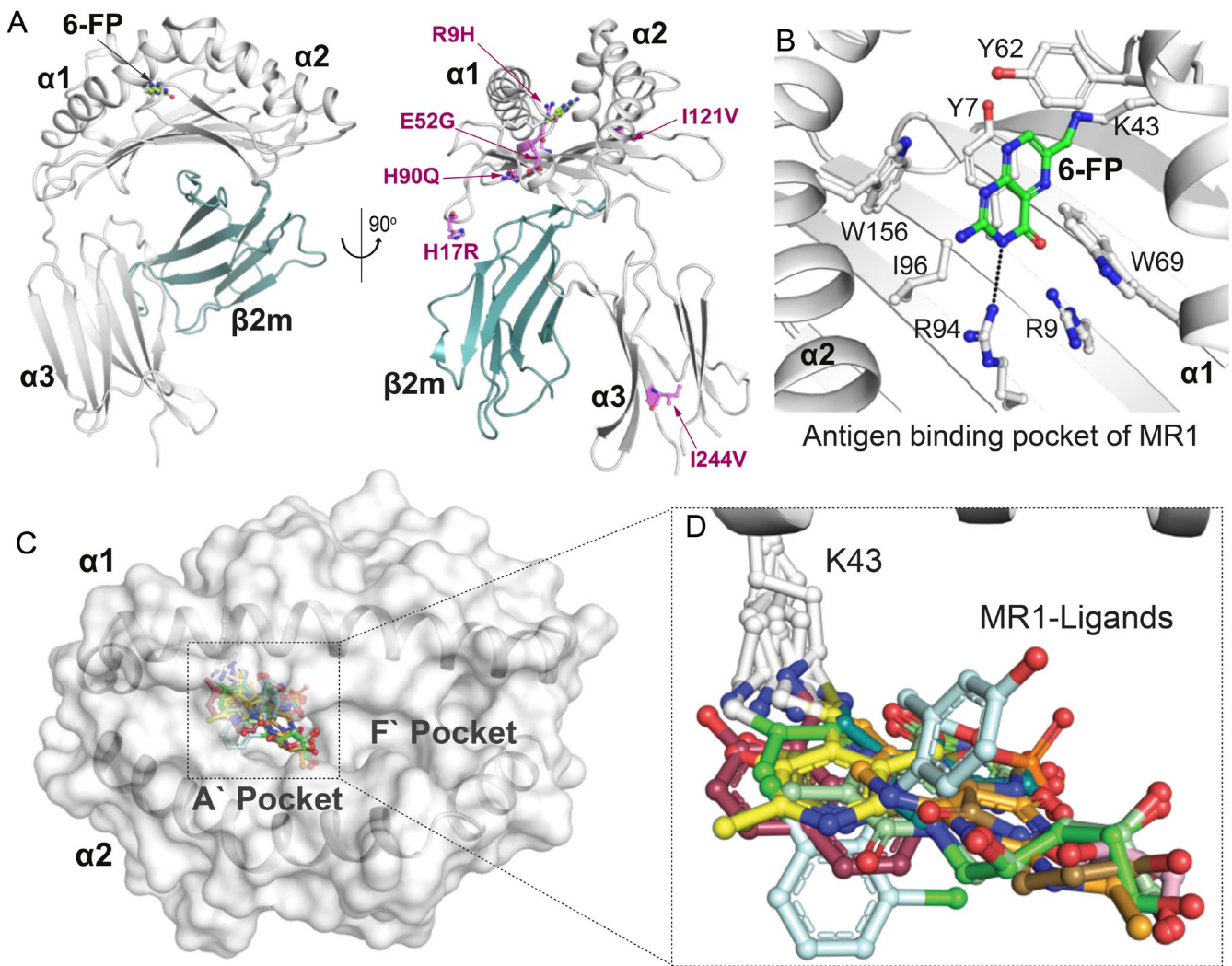
FIGURE 1 | Crystal structure of MR1-Ags. (A) Cartoon presentation of the structure of the binary MR1-6-FP complex (PDB; 6GUP). MR1 and \beta 2m, and 6-FP ligand are colored white, gray, and green, respectively. Mutations in various MR1 alleles are shown in pink. (B) The interactions of 6-FP within the A'-pocket of the MR1 binding cleft. MR1-Ag interacting residues are shown as white sticks, and the H-bond is shown as a black dashed line. (C) Surface presentation of the MR1-Ag binding A' and F' pockets that are formed between MR1 \alpha 1 and \alpha 2 helices. All recognized MR1-ligands, to date, dock in the A' pocket as shown in (D).
