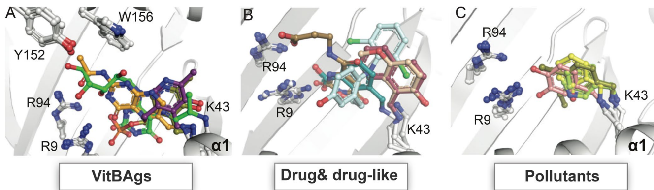
FIGURE 3 | MR1 presentation of small metabolites. Superimpositions of the Ag binding pocket of MR1 binding: (A) VitBAGs: 5-OP-RU; (PDB: 6PUC), Ac-6-FP (PDB: 4PJ5); PL (PDB: 9CGR); and PLP (PDB: 9CGS), (B) Drug and drug-like Ags: 5-OH-DCF (PDB: 5U72); HMB (PDB: 5U2V); 3-F-SA (PDB: 5U6Q); 2-OH-1-NA (PDB: 5U16) and DB28 (PDB: 6PVC), (C) Pollutants ligands: Salicylaldehyde (PDB: 9BU0); veratraldehyde (PDB: 9BTY); nicotinaldehyde (PDB: 9BTZ); and 3,4-dihydroxybenzaldehyde (PDB, 9BTX). MR1-ligands are represented as colored sticks.
