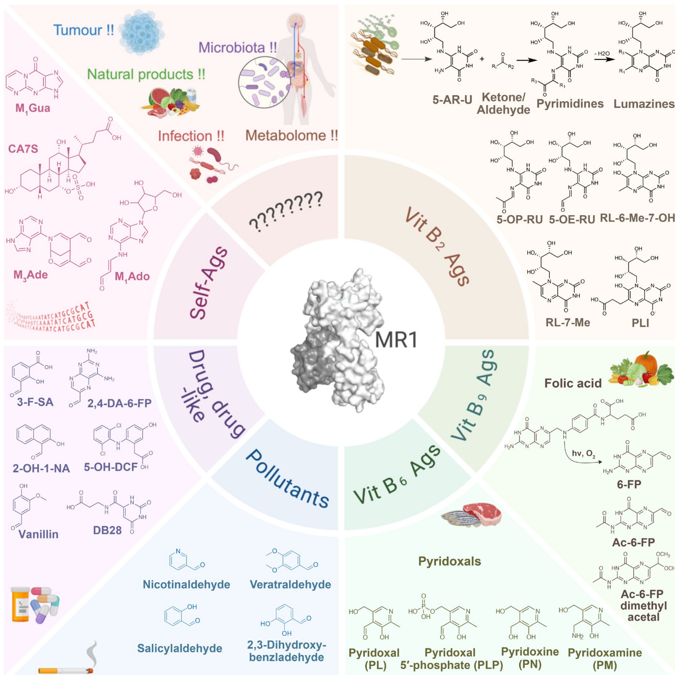
FIGURE 2 | Schematic of various categories of MR1 ligands, including microbial and non-microbial derived VitB 6 , drug, drug-like, environmental, and self-antigens.
