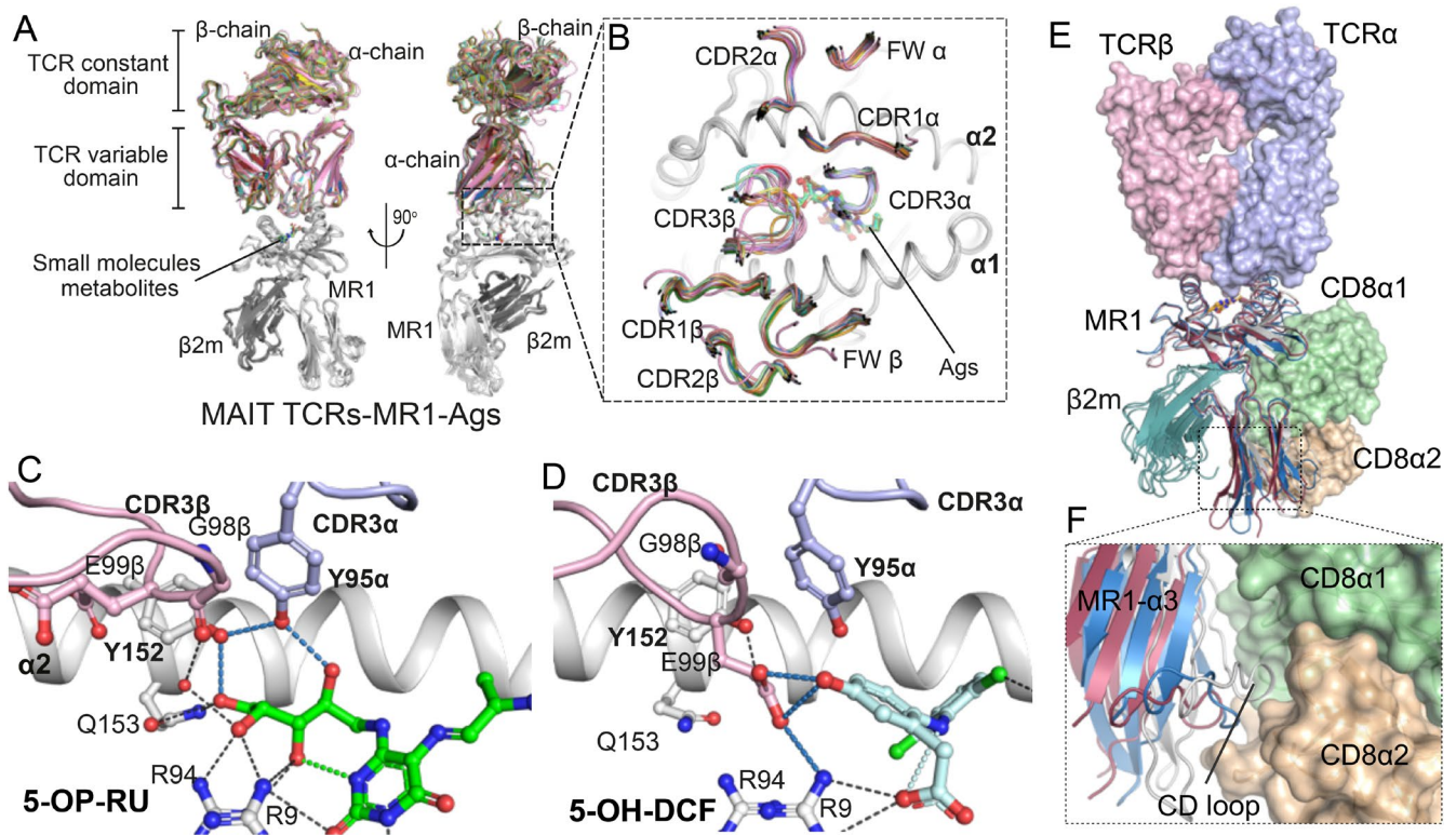
FIGURE 4 | TCR-MR1-Ag “Interaction Triad” formation with MAIT agonists. (A) Superimposition of the MAIT TRAV1-2 pos TCR-MR1-Ags structures with zooming into the top view of the Ag-binding cleft of the respective MR1 molecule, displaying similar docking of the TCR CDR loops atop the MR1 molecule (B). (C) MAIT TCR-MR1-Ag interaction triad (encompassing the 5-OP-RU, TCR-Tyr95α, and MR1-Tyr152). (D) Recognition of 5-OH-DC by classical MAIT AF-7 TCR. CDR3α and CDR3β are colored light blue and light pink, respectively. (E) Superimposition of the binary MR1-6FP, CD8αα-MR1-Ac-6-FP, and MAIT-TCR-MR1-Ac-6-FP complexes. (F) Zoomed view of the interaction between CD8αα and the CD loops of the α3 domains of MR1. MR1 molecules were shown as colored ribbons, and TCR and CD8αα were shown as surface representations.
