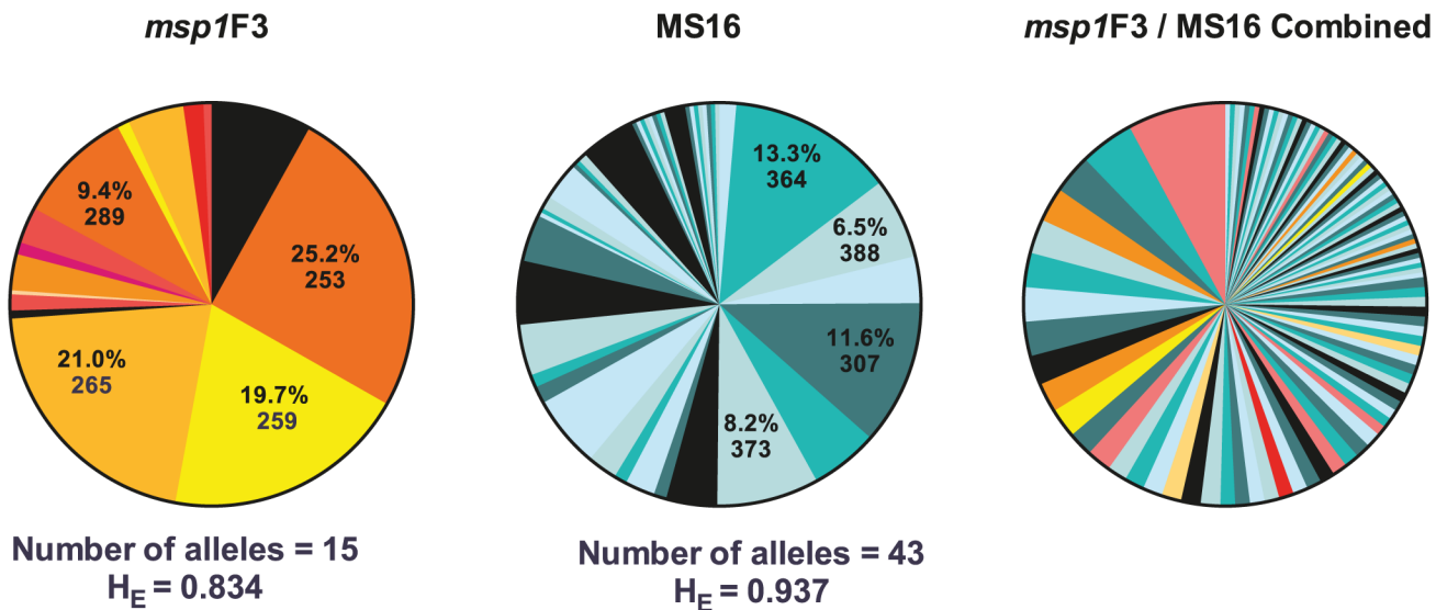
Fig 3. Diversity of P. vivax genotypic markers msp1F3 and MS16 . Allelic frequencies of P. vivax msp1F3 , MS16 and the combined msp1F3 / MS16 haplotypes. For msp1F3 and MS16 , the frequency of the four most common alleles and respective sizes (in basepairs) are shown. The number of unique alleles identified and the estimated expected heterozygosity ( H_E ) are given below the figure.
