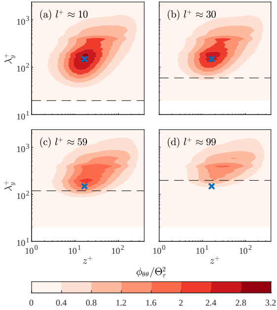
Figure 4. Pre-multiplied one-dimensional energy spectra of the temperature fluctuation ( \Phi_{00}/\Theta_\tau^2 ) as a function of \lambda_y^+ against wall distance with different filter length (a) l^+ \approx 10 (unfiltered), (b) l^+ \approx 30 , (c) l^+ \approx 59 and (d) l^+ \approx 99 . \times is marked at \lambda_y \approx 110 at location of z^+ \approx 18 . The horizontal dashed line shows \lambda_y^+ = 2l^+ .
