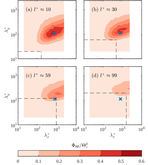
Figure 5. Pre-multiplied two-dimensional energy spectra of temperature ( \Phi_{00}/\Theta_\tau^2 ) as a function of streamwise wavelength ( \lambda_x ) and spanwise wavelength ( \lambda_y^+ ) with filter length (a) l^+ \approx 10 (unfiltered), (b) l^+ \approx 30 , (c) l^+ \approx 59 and (d) l^+ \approx 99 at the wall-normal location of z^+ \approx 18 . \times is marked at \lambda_x^+ \approx 800 and \lambda_y^+ \approx 110 . The horizontal dashed line shows \lambda_y^+ = 2l^+ and the vertical dashed line shows \lambda_x^+ = 16l^+ .
