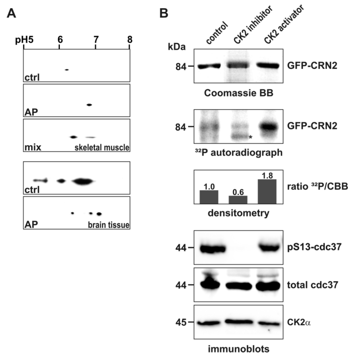
Figure 4 | CK2 phosphorylates CRN2 in vivo . (A) presence of a phosphorylated pool of endogenous CRN2. Lysates of murine skeletal muscle (upper three panels) and brain tissue (lower two panels) were separated by 2D-gel electrophoresis. CRN2 was visualized by western blotting using mAb K6-444. The first panel presents the untreated sample (ctrl), the second panel the in vitro de-phosphorylated sample (alkaline phosphatase, AP), and the third panel shows two CRN2 spots resulting from a mixture of the untreated and de-phosphorylated samples (muscle sample only). In contrast to brain tissue (fourth and fifth panel), in skeletal muscle only a single spot of CRN2 is detected which corresponds to CRN2 isoform 3 5 . (B) modulation of the in vivo CK2 activity changes the phosphorylation status of CRN2. 293TN cells over-expressing GFP-CRN2 were grown in the presence of the CK2 inhibitor TBB, the CK2 activator 1-ethyl-4,5-dicarbamoylimidazole or solvent control before addition of 32 P-orthophosphate. Subsequently, cells were lysed, GFP-CRN2 was immunoprecipitated, samples were separated by SDS-PAGE, proteins were stained by Coomassie brilliant blue (first panel), and gels were dried and used for autoradiography (second panel). Densitometric analysis determined that the CK2 inhibitor decreased the level of CRN2 phosphorylation by 40%, while application of the activator led to an increase of 80% (third panel). Immunoblots for pS13-cdc37, a marker of the in vivo CK2 activity, total cdc37, and CK2α are given as controls (fourth to sixth panel). One representative experiment is shown. First and second panel, for illustration purposes the order of lines from the original data was digitally re-arranged. Asterisk, unspecific autoradiography signal which does not correspond to the Coomassie stained CRN2 protein band.
