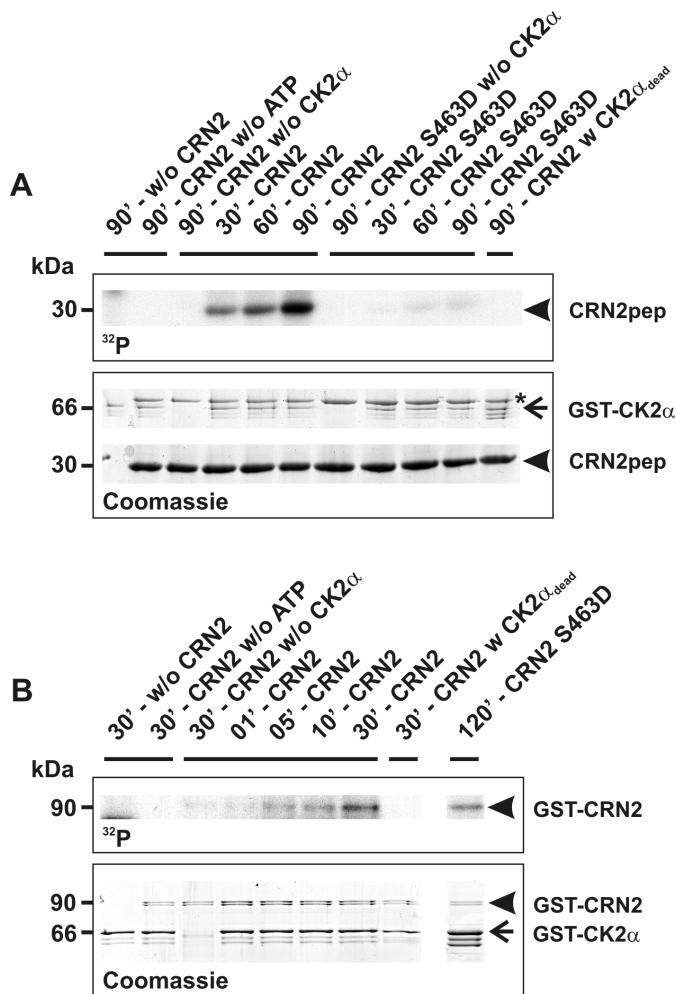
Figure 3 | CRN2 is a target of CK2α and is phosphorylated at S463. (A) in vitro kinase assays employing recombinant full-length GST-CK2α (66 kDa, arrow) and His-tagged C-terminal polypeptides of CRN2 (30 kDa, arrowheads). Time course (30, 60, 90 minutes) of phosphate incorporation from [ \gamma - 32 P]ATP into wild-type as well as S463D mutant CRN2 polypeptides. Controls where the CRN2 polypeptide, [ \gamma - 32 P]ATP, or CK2α were omitted and use of a kinase-dead CK2α are indicated. Upper panel, autoradiograph of phosphorylation of CRN2 ( 32 P). Lower panel, the corresponding Coomassie brilliant blue stained gel. For all lines containing CK2α identical volumes from the same preparation of purified enzyme were used. Molar concentrations, CK2α 30 nM, CRN2 1.8 μM. Asterisk, contamination by the E. coli 70 kDa chaperone DnaK. Wild-type CRN2 is phosphorylated in a time-dependent manner. Note the minor phosphorylation levels of the mutant polypeptide after 90 min. (B) in vitro kinase assay employing recombinant full-length GST-CK2α (66 kDa, arrow) and GST-His-tagged full-length CRN2 purified from insect cells (90 kDa, arrowheads). Time course (1, 5, 10, 30 minutes) of phosphate incorporation from [ \gamma - 32 P]ATP into wild-type CRN2. Controls where CRN2, [ \gamma - 32 P]ATP, or CK2α were omitted and use of a kinase-dead CK2α are indicated. Upper panel, autoradiograph of phosphorylation of CRN2 ( 32 P). Lower panel, the corresponding Coomassie brilliant blue stained gel. For all lines containing CK2α identical volumes from the same preparation of purified enzyme were used. CRN2 is phosphorylated in a time-dependent manner. Note, that only after longer incubation time (120 min) the phosphorylation level of S463D mutant CRN2 reaches the one of wild-type CRN2.
