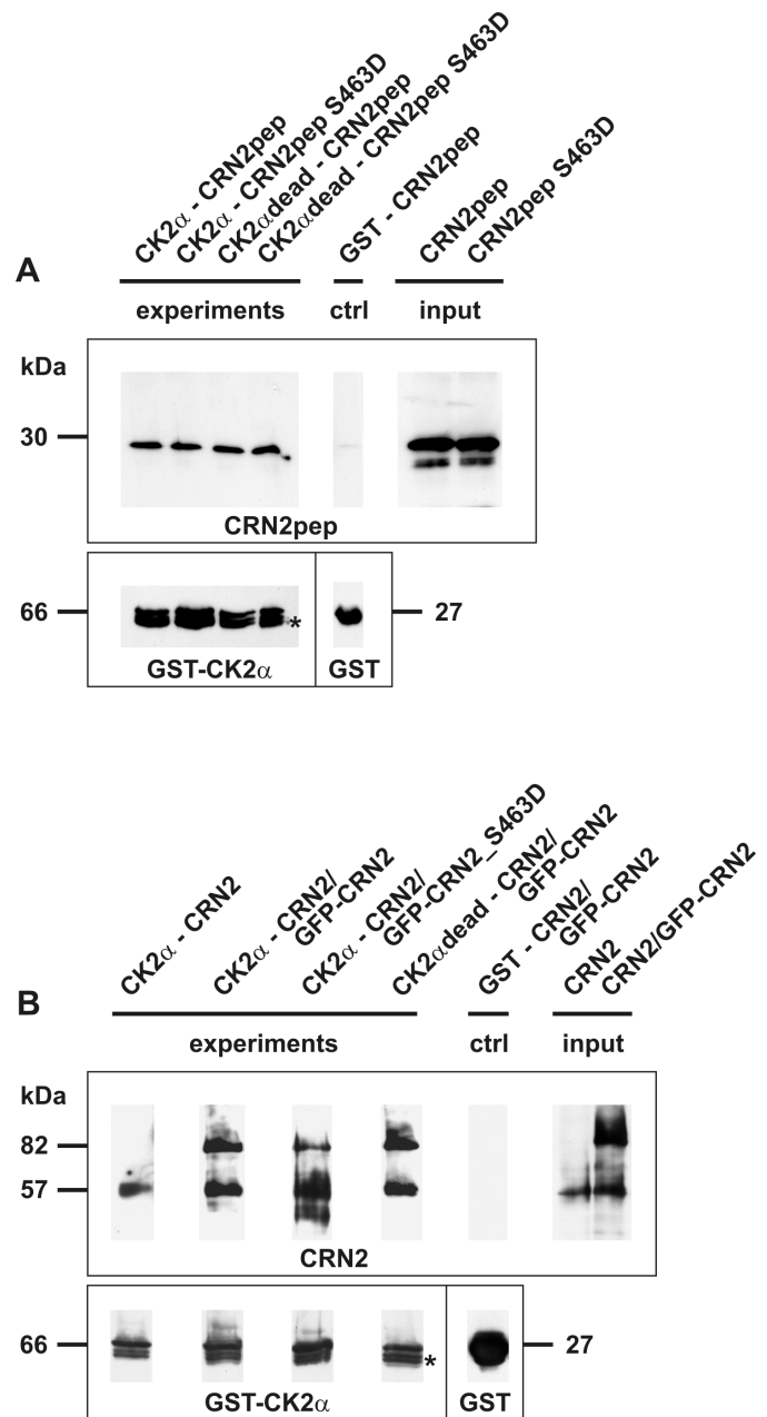
Figure 2 | CRN2 directly interacts with CK2 \alpha . (A) pull-down assay employing purified recombinant full-length GST-tagged CK2 \alpha coupled to glutathione beads and purified soluble CRN2 wild-type and phosphomimetic S463D C-terminal polypeptides (aa300-474). Both polypeptides bind to CK2 \alpha and CK2 \alpha dead, the latter lacks kinase activity. (B) pull-down assay employing purified recombinant full-length GST-tagged CK2 \alpha coupled to glutathione beads and lysates from HEK293 cells over-expressing endogenous CRN2 (57 kDa) as well as GFP-CRN2 (82 kDa) fusion proteins. Endogenous, wild-type GFP-CRN2, and GFP-CRN2 S463D bind to CK2 \alpha . All CRN2 polypeptides were detected with antibody K6-444, and GST-CK2 \alpha immunoblotting was done with a rabbit polyclonal GST-antibody 86 . Asterisk, two additional CK2 \alpha bands are the result of degradation. Controls contained beads coated with GST alone. For illustration purposes individual lines from the original western blots were digitally re-arranged.
