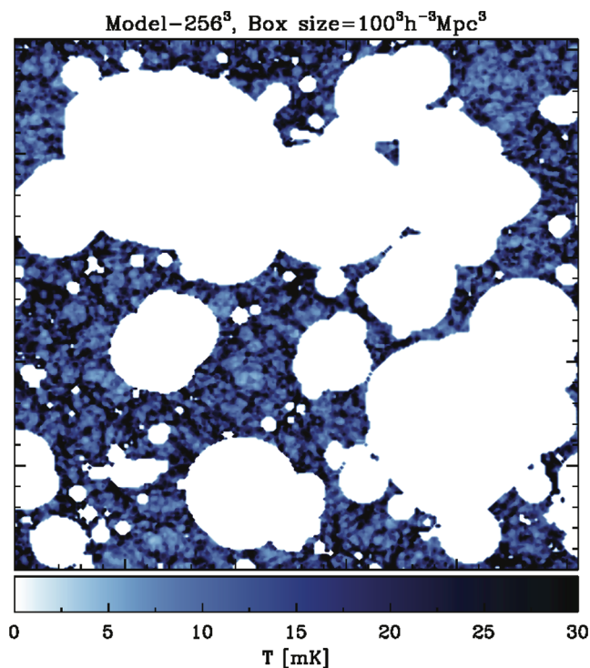
Figure 3. The 21-cm intensity map from the Model-256 3 (cell size 0.39 Mpc h^{-1} ) at z \sim 7.272 ( \langle x_i \rangle \sim 0.55 ) with slice that is 0.39 Mpc h^{-1} deep. The colour shading shows the 21-cm intensity in temperature units, as indicated by the bar.
