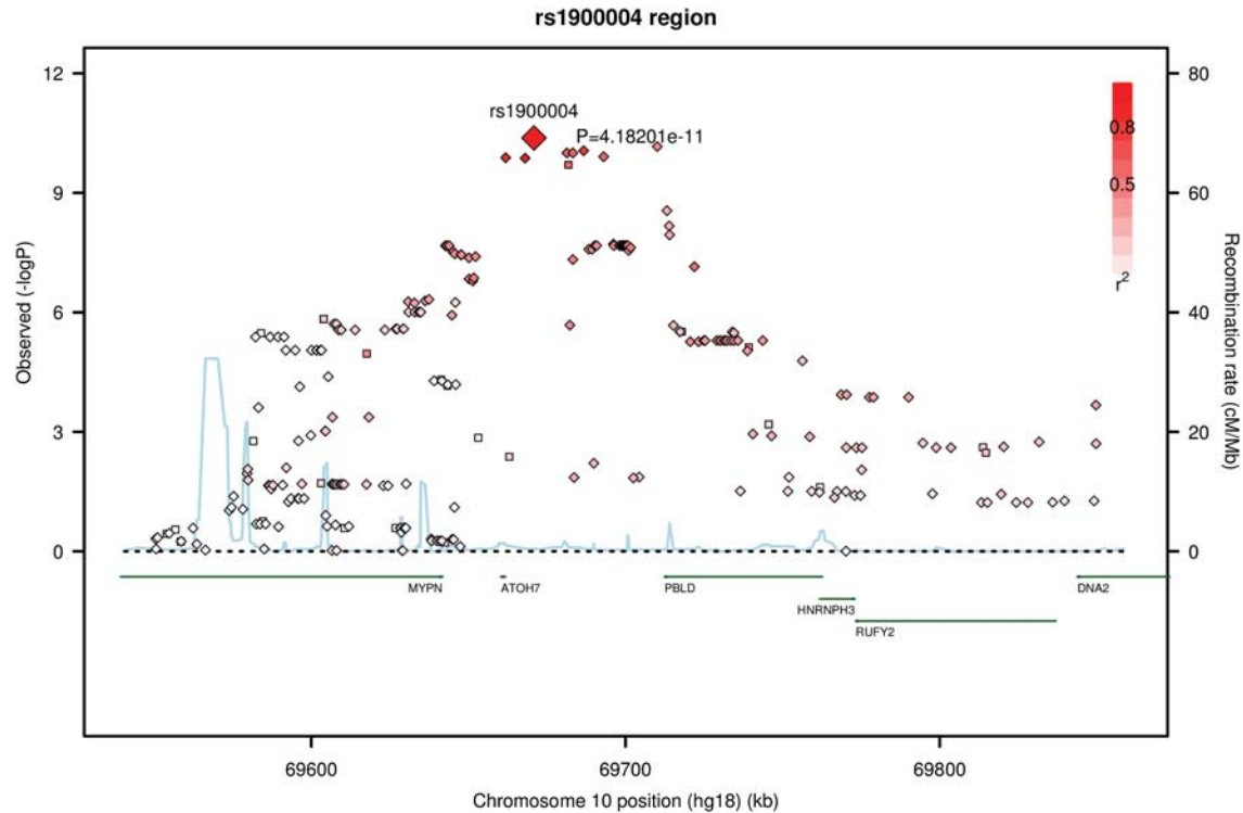
Figure 3. Significant association of the optic nerve endophenotype disc area at the chromosome 10q21 locus. Results from the meta-analysis of both the Australian and UK twin cohorts are presented. Imputed SNPs are indicated by diamonds and genotyped SNPs by squares. The degree of linkage disequilibrium between rs1900004 and other SNPs is indicated by red shading. The recombination rate is displayed in light blue line, with scale on the right-hand axis.
