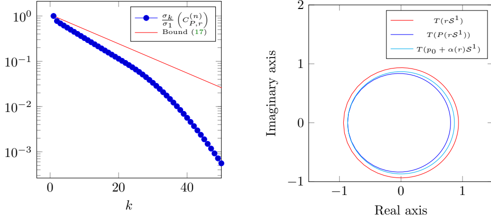
FIG. 7. Case p_0 = 0.55 . On the left, the first relative singular values of C_{P,r}^{(n)} , with n = 1000 , compared with the bound in (17). On the right, the image of the regions r\mathcal{S}^1 , P(r\mathcal{S}^1) and p_0 + \alpha(r)\mathcal{S}^1 under the Möbius transformation T(z) = (z - \alpha)/(z - \beta)
