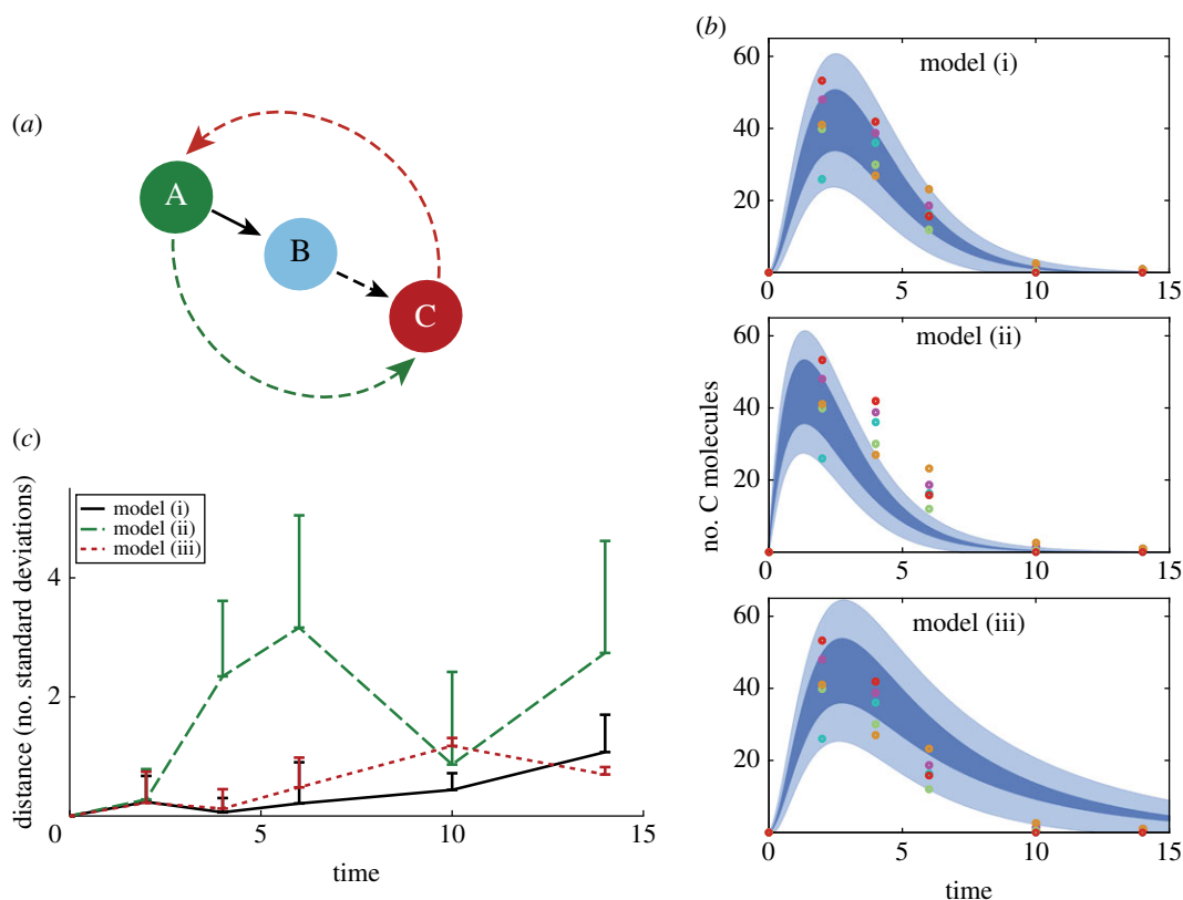
Figure 2. Model evaluation by comparing reachable sets and single measurements. (a) Schematics of the three reaction chain models. Models differ in rates corresponding to dashed arrows. (i) k_{BC} = 1 , k_{AC} = k_{CA} = 0 . (ii) k_{BC} = 0.1 , k_{AC} = 0.9 , k_{CA} = 0 . (iii) k_{BC} = 1 , k_{AC} = 0 , k_{CA} = 0.2 . (b) Reachable region over time of the output (molecule C) starting from the initial set 80 \leq A_0 \leq 120 , B_0 = C_0 = 0 . Dark areas represent reachable values of the mean, light blue shades are the \pm 1 s.d. region computed with the maximal reachable value of the variance. Coloured circles are sample points taken from single exact simulations of model (i). (c) Distance of observation points from the reachable set of mean values. Lines show the average distance of observed data points at each time of measurement, the top of error bars depict the maximal distance at the evaluation points (colours as indicated in legend). Distances for each model are normalized by the maximal reachable standard deviation value. Time in (b) and (c) is in arbitrary units based on the macromolecular production rate, such that with maximal interaction strength, on average one product molecule is created in 1 t.u.
