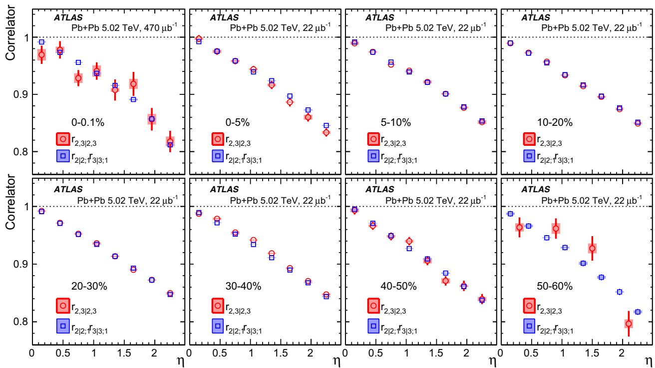
Fig. 21 The r_{2,3|2,3} (circles) and r_{2|2;1}r_{3|3;1} (squares) as a function of \eta for several centrality intervals. The error bars and shaded boxes are statistical and systematic uncertainties, respectively. The r_{2,3|2,3} data in the 50–60% centrality interval are rebinned to reduce the uncertainty
