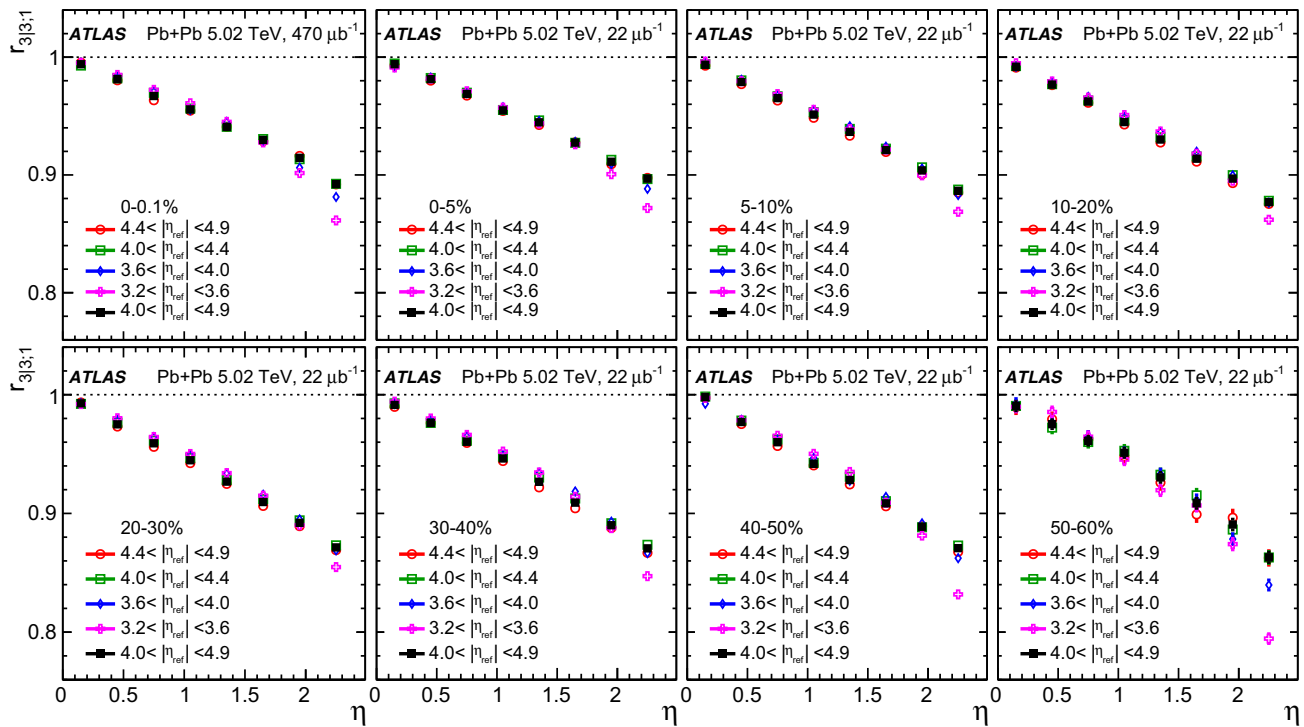
Fig. 3 The r_{3|3;1}(\eta) measured for several \eta_{\text{ref}} ranges. Each panel shows the results for one centrality range. The error bars are statistical only
