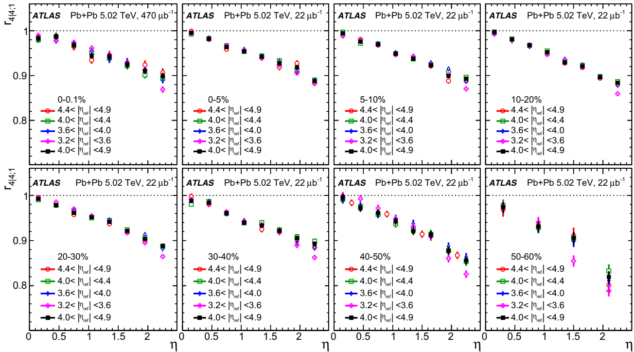
Fig. 27 The r_{4|4;1}(\eta) measured for several \eta_{\text{ref}} ranges for Pb+Pb collisions at 5.02 TeV. Each panel represents one centrality range. The error bars are statistical only. The data points in some centrality intervals are rebinned to reduce the uncertainty
