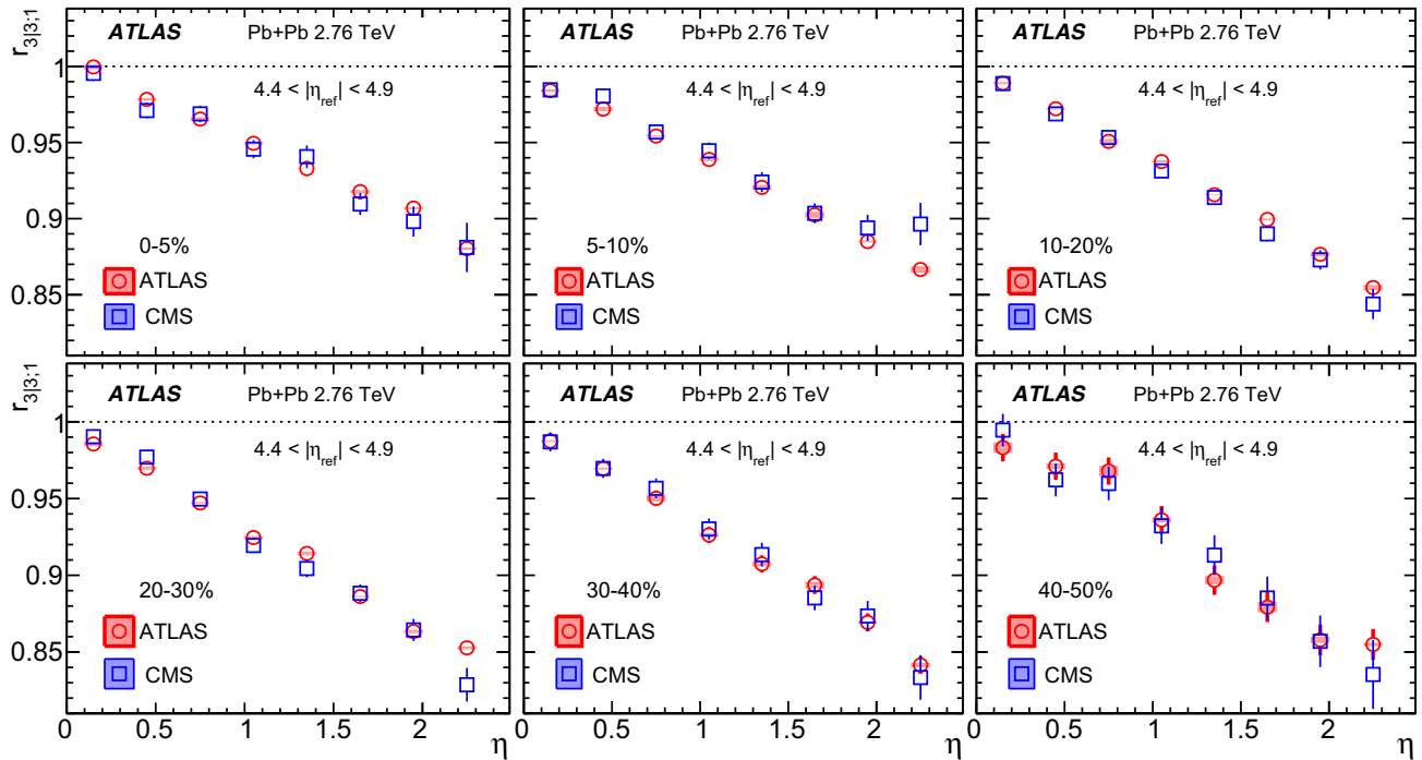
Fig. 26 The values of r_{3|3;1} measured by ATLAS and by CMS [19] for Pb+Pb collisions at 2.76 TeV, for the same reference pseudorapidity 4.4 < |\eta_{\text{ref}}| < 4.9
