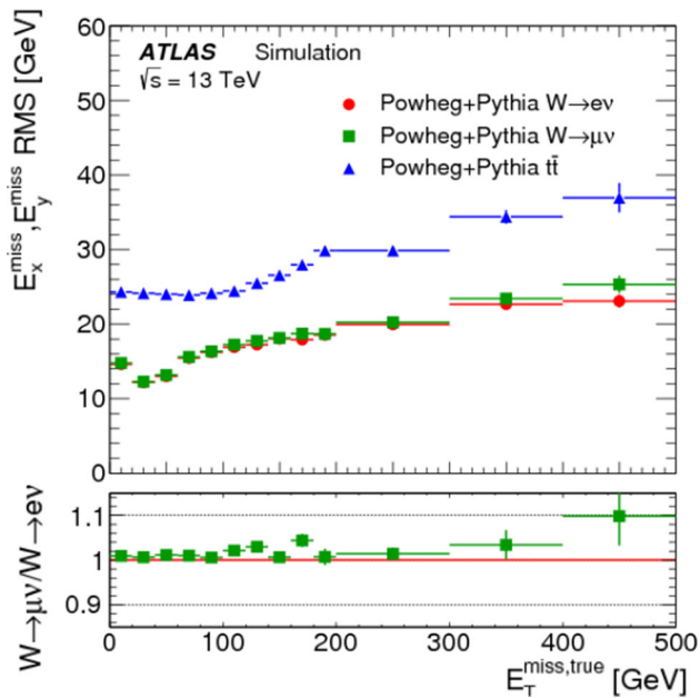
Fig. 9 The E_T^{\text{miss}} resolution measured by \text{RMS}_{x(y)}^{\text{miss}} as a function of the true missing transverse momentum E_{T,\text{true}}^{\text{miss}} for the W \rightarrow e\nu , W \rightarrow \mu\nu , and t\bar{t} samples from MC simulations
