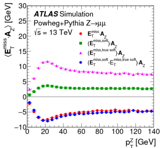
Fig. 5 The average projection of E_T^{\text{miss}} onto the direction A_Z of the Z boson's transverse momentum vector p_T^Z , as given in Eq. (10), is shown as a function of p_T^Z = |p_T^Z| in Z \rightarrow \mu\mu events from the inclusive MC sample. The average projection of the soft term and the true soft term are also shown, to demonstrate the source of the deviation from zero
