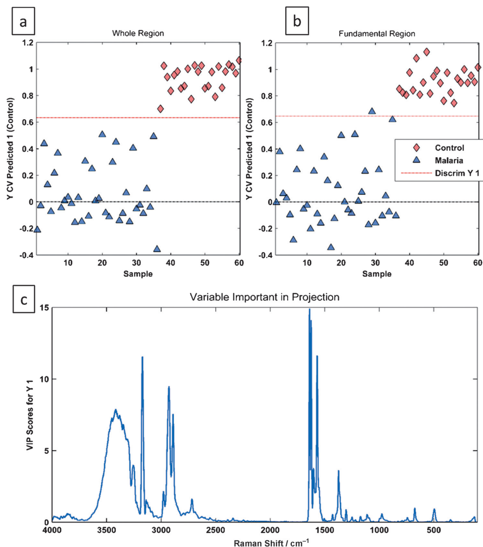
Figure 4. Cross-validation errors for the PLS-DA performed on the evaluation of the discrimination capability between the control (non-infected RBCs) and malaria (infected RBCs) samples, using the whole (a) and the fundamental (b) regions. Variable importance in projection for the PLS-DA performed on the whole region (c).
