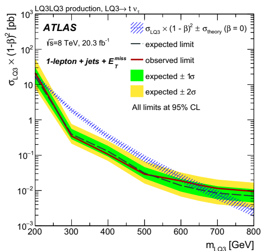
Fig. 6 The expected (dashed) and observed (solid) 95 % CL upper limits on the third-generation scalar LQ pair-production cross-section times the square of the branching ratio to t\nu_\tau as a function of LQ mass, for the t\nu_\tau\bar{t}\bar{\nu}_\tau channel. The \pm 1(2)\sigma uncertainty bands on the expected limit represent all sources of systematic and statistical uncertainty. The expected NLO production cross-section ( \beta = 0.0 ) for third-generation scalar LQ pair-production and its corresponding theoretical uncertainty due to the choice of PDF set and renormalisation/factorisation scale are also included
