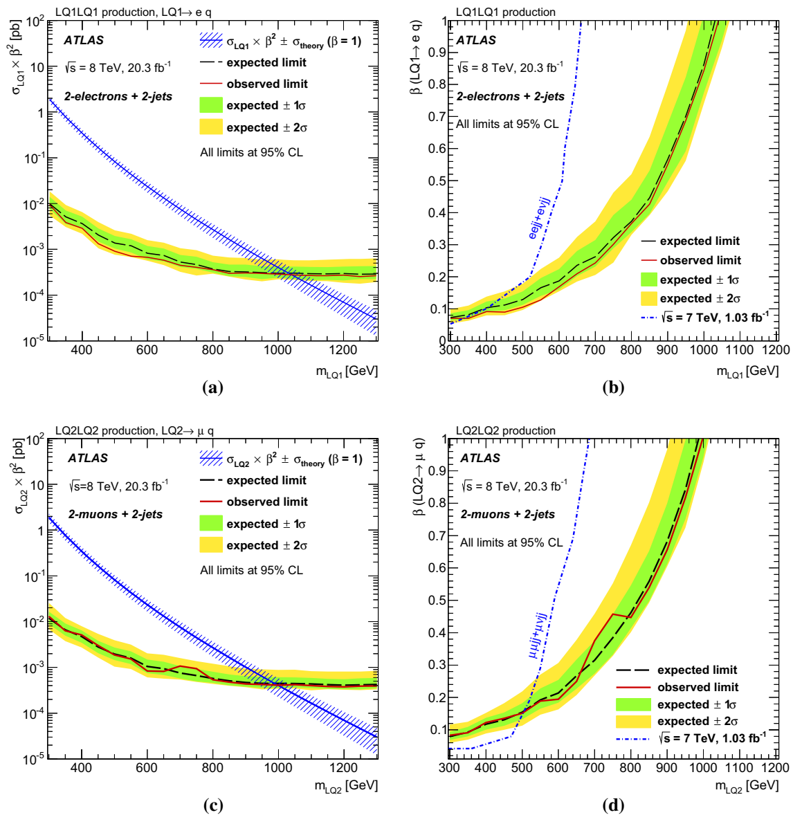
Fig. 4 The cross-section limits on scalar LQ pair-production times the square of the branching ratio as a function of mass ( left ) and the excluded branching ratio as a function of the LQ mass ( right ) to eq for the eejj channel ( top ) and to \mu q for the \mu\mu jj channel ( bottom ). The \pm 1(2)\sigma uncertainty bands on the expected limit represent all sources of systematic and statistical uncertainty. The expected NLO production
