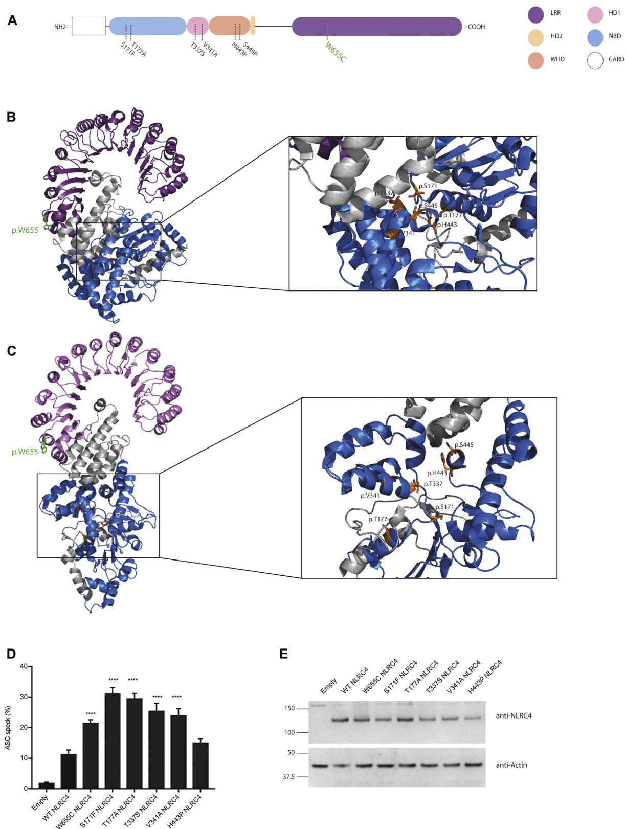
FIG 4. p.W655 is located in the LRR domain of NLRC4. A , Schematic representation of NLRC4 domains, with the variant of interest shown in green. B and C , Ribbon representation of secondary structure of autoinhibited (PDB Code 4KXF 23 ; Fig 4, B ) and active (PDB Code 6B5B 24 ; Fig 4, C ) NLRC4. p.W655C NLRC4 is displayed in stick format in green. D and E , ASC speck quantification of WT and NLRC4 mutants by using flow cytometry (Fig 4, D ), with NLRC4 expression in whole-cell lysate assessed by using Western blotting (Fig 4, E ). Data are pooled from 5 independent experiments: * P < .05 , ** P < .01 , *** P < .001 , and **** P < .0001 . NBD, Nucleotide binding domain; WHD, winged helix domain.
