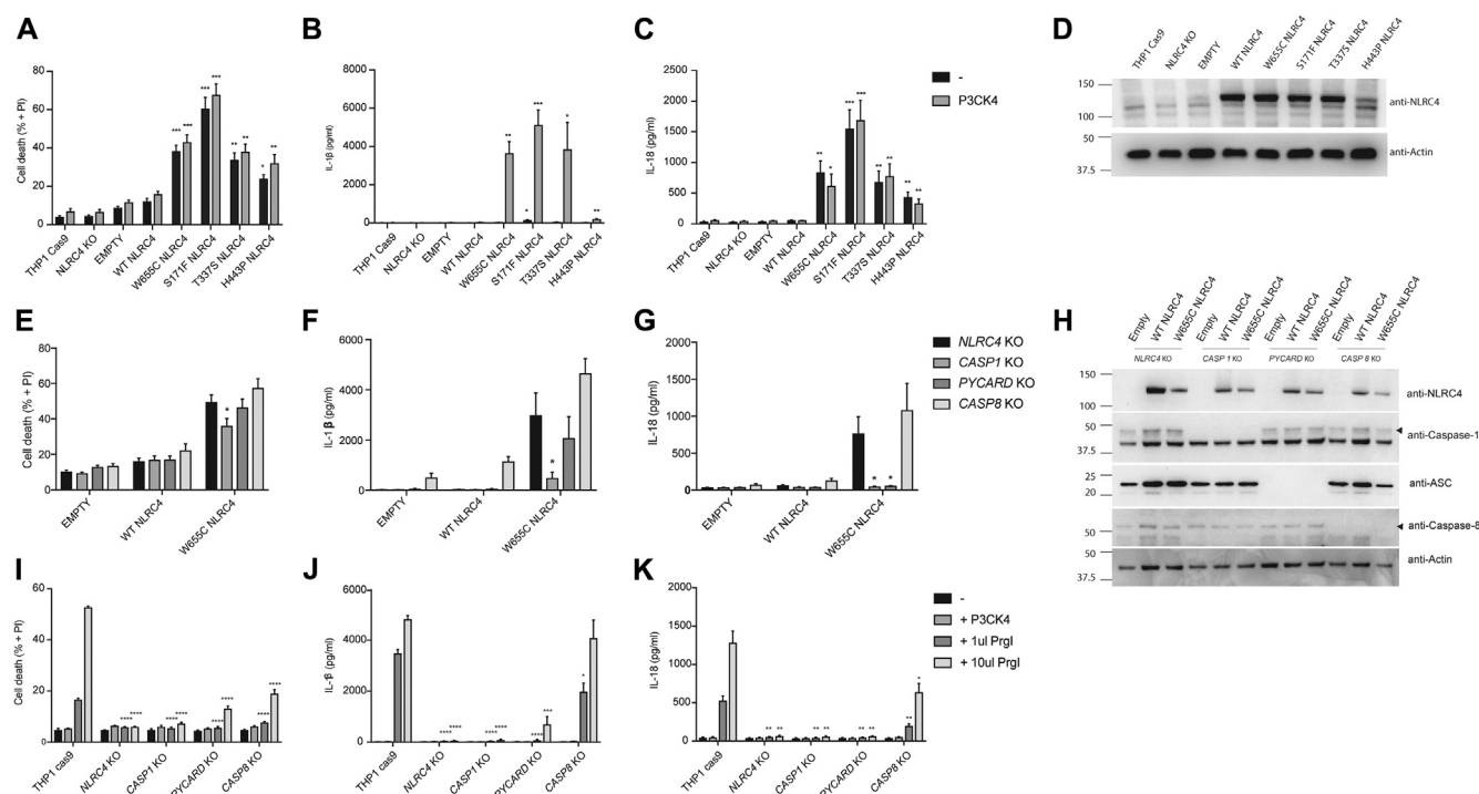
FIG 5. Effects of p.W655C NLRC4 on cytokine production and cell death. NLRC4 KO THP-1 monocytes were transduced with lentivirus coding for WT or various NLRC4 mutations (as indicated). Twenty-four hours after transduction, cells were plated and treated with Pam3CSK4. A-C , After 24 hours, propidium iodide (PI) staining was assessed by using flow cytometry to quantify cell death (Fig 5, A), and IL-1 \beta (Fig 5, B) and IL-18 (Fig 5, C) secretion was measured by means of ELISA. D , Expression of NLRC4 under each condition was qualified by means of Western blotting of whole-cell lysates. E-H , CASPASE1 , PYCARD , or CASPASE8 KO THP-1 monocytes were transduced with WT or p.W655C NLRC4 , and assessment of cell death (Fig 5, E) and IL-1 \beta (Fig 5, F) and IL-18 (Fig 5, G) secretion was undertaken after treatment with Pam3CSK4, with expression of NLRC4 determined by using Western blotting (Fig 5, H). THP-1 cells, along with NLRC4 , CASPASE1 , PYCARD , or CASPASE8 KO THP-1 monocytes, were primed for 3 hours with Pam3CSK4 and infected with 2 amounts of retrovirus expressing PrgI needle protein. I-K , After 24 hours, cell death (Fig 5, I) and IL-1 \beta (Fig 5, J) and IL-18 (Fig 5, K) secretion were assessed with flow cytometry and ELISA, respectively. Data were pooled from at least 3 independent experiments. * P < .05 , ** P < .01 , and *** P < .001 .
