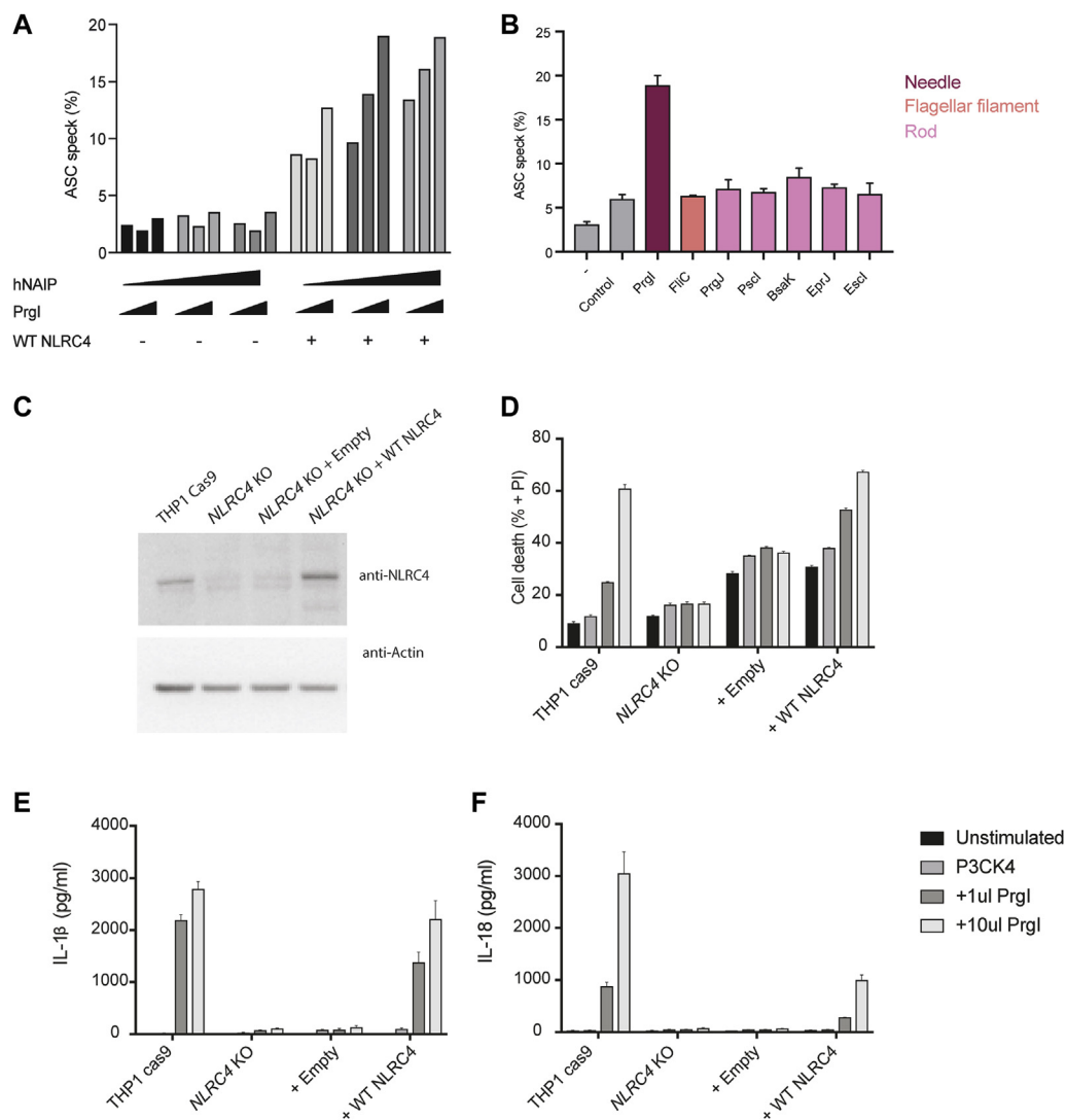
FIG E2. T3SS selection and validation of NLRC4 KO THP-1 cells. HEK293T cells were transfected with WT NLRC4 , as well as increasing amounts of human NAIP ( hNAIP ) and the T3SS needle protein Prgl. A , Flow cytometric analysis of ASC speck formation shows that WT NLRC4 is needed for ASC speck formation and that hNAIP is required for ASC specks to increase in response to low amounts of Prgl. B , Various T3SS proteins were transfected into HEK293T cells in addition to WT NLRC4 and hNAIP to ensure specificity of response. The ASC speck response is specific to the only needle protein tested, Prgl. C , THP-1-Cas9 cells infected with inducible single guide RNA targeting exon 2 of NLRC4 were treated with doxycycline for 72 hours and expression of NLRC4 assessed with Western blotting performed on whole-cell lysates after 48 hours of rest. Cells were then primed with Pam3CSK4 and infected with 2 amounts of retrovirus expressing Prgl needle protein. D-F , After 24 hours of assessment of cell death (Fig E2, D ), IL-1 \beta (Fig E2, E ) and IL-18 (Fig E2, F ) secretion was undertaken.
