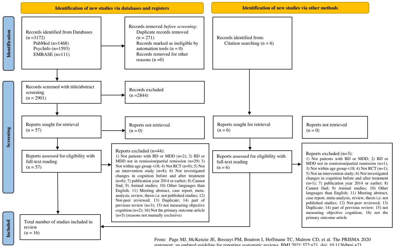
FIGURE 1 PRISMA 2020 flowchart
