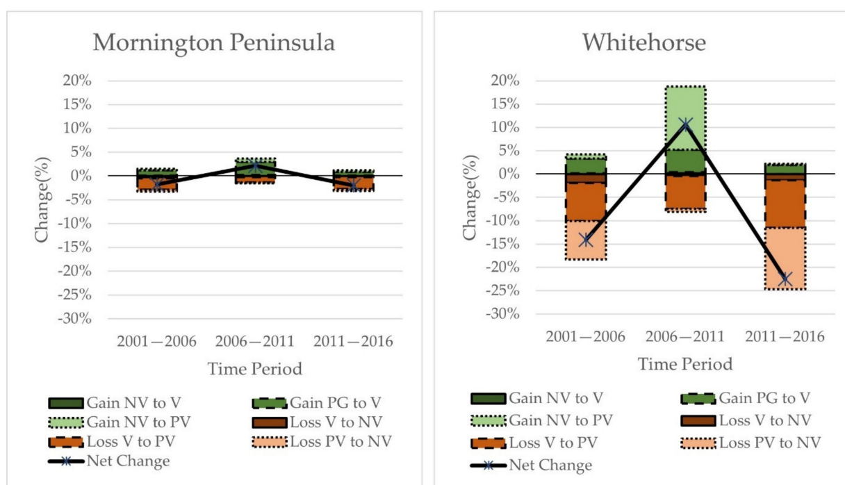
Figure 3. Pattern of change in urban vegetation over 15 years. The change has been shown over three time periods—T1 (2001 to 2006), T2 (2006 to 2011) and T3 (2011 to 2016). Net change and six processes of change have been included in the study, including: (1) gain from non-vegetated to vegetated (Gain NV to V), (2) gain from partially vegetated to vegetated (Gain PV to V), (3) gain from non-vegetated to partially vegetated (NV to PV), (4) loss from vegetated to non-vegetated (Loss V to NV), (5) loss vegetated to partially vegetated (Loss V to PV) and (6) loss from partially vegetated to non-vegetated (PV to NV). Among these six processes of changes, the gain (1) and losses (4) involving changes between non-vegetated (NG) and vegetated (G) pixels are referred to as absolute changes, whereas the other four processes (2, 3, 5, 6) are referred as potential changes.
