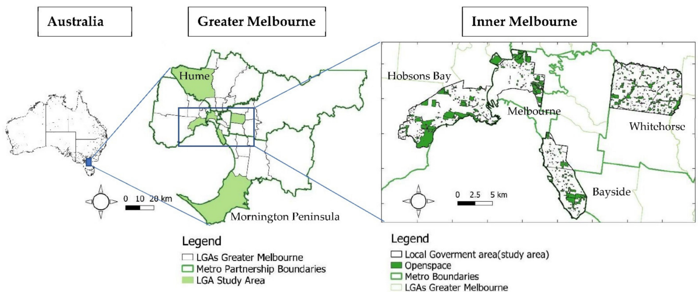
Figure 2. Study area showing Greater Melbourne with six local government areas (middle) and open space in four LGAs in Inner Melbourne (right). The location of Melbourne within Australia is shown in the left panel.
