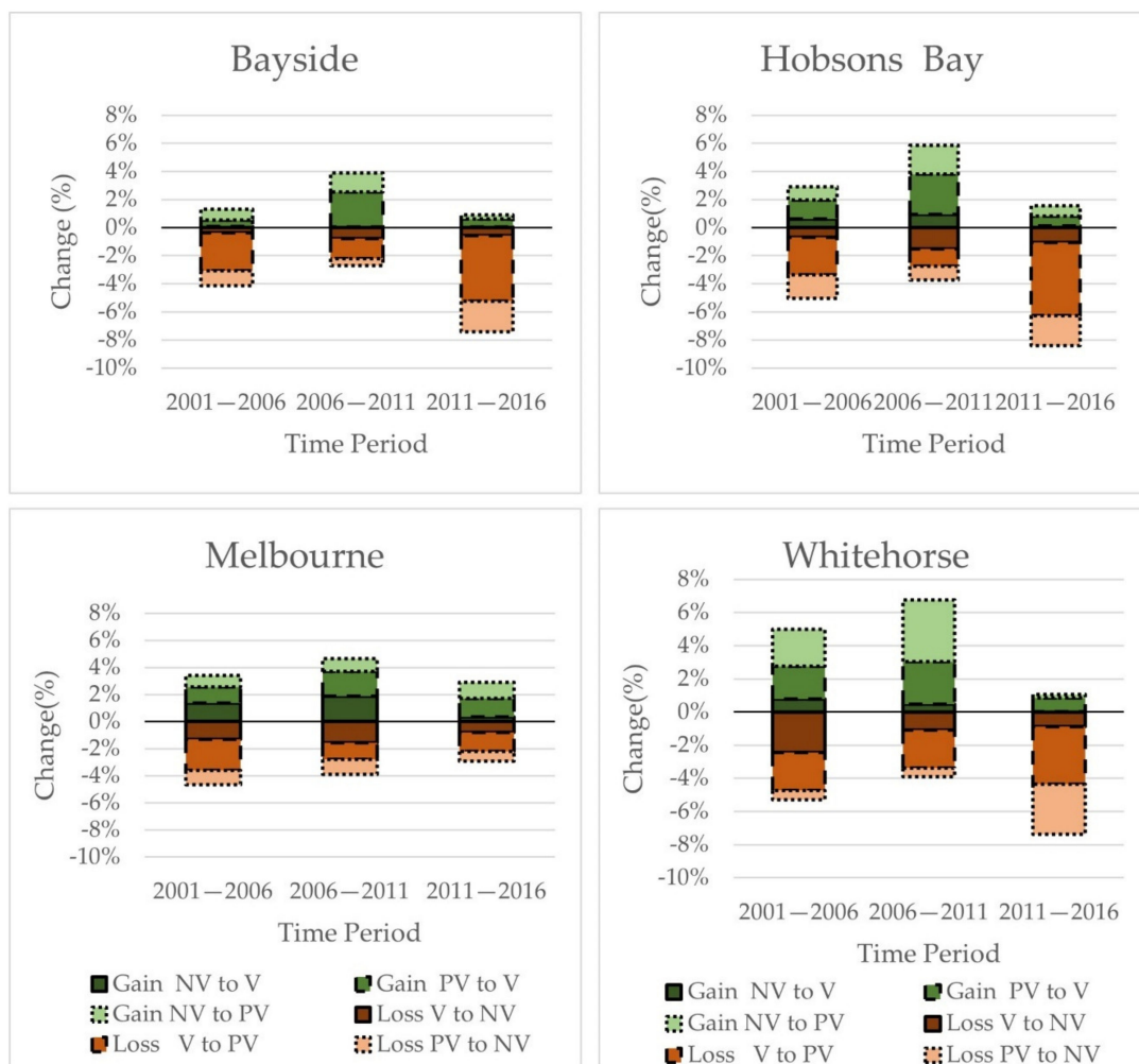
Figure 4. Pattern of change of vegetation within public open space features over a fifteen-year period. The change was calculated for three periods: T1 (2001 to 2006), T2 (2006 to 2011) and T3 (2011 to 2016). Six processes of change were included in the study: (1) gain from non-vegetated to vegetated (Gain NV to V), (2) gain from partially vegetated to vegetated (Gain PV to V), (3) gain from non-vegetated to partially vegetated (NV to PV), (4) loss from vegetated to non-vegetated (Loss V to NV), (5) loss from vegetated to partially vegetated (Loss V to PV) and (6) loss from partially vegetated to non-vegetated (PV to NV). Among six processes of changes, the gain (1) and losses (4) involving changes between non-vegetated (NV) and vegetated (V) pixels are referred to as absolute changes, whereas the other four processes (2, 3, 5, 6) are referred as potential changes.
