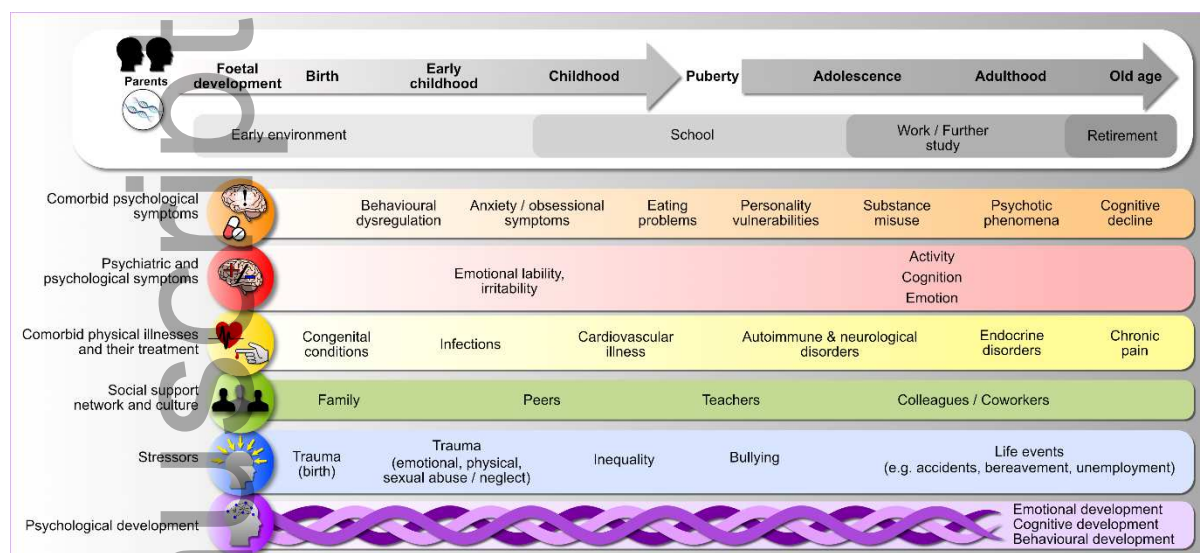
Figure 2. A framework for assessing the clinical factors that contribute to depression.
