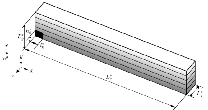
Fig. 1: Sketch of initial condition of the simulation. The black represents the dense fluid ( \rho_c ) and h_0 and l_0 are the height and length of the dense fluid. The density of the fluid at the top, \rho_0 (white) is increased linearly to \rho_b (grey) at the bottom of the domain where L_x^* , L_y^* and L_z^* are the streamwise length, wall-normal length and span-wise length of the domain.
