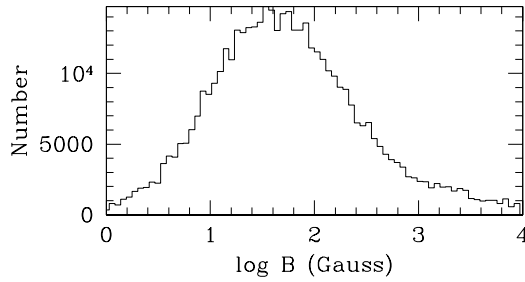
Fig. 6 Predicted magnetic field distribution of massive stars ( 8 - 45 M_{\odot} ), according to the population synthesis modelling of Ferrario and Wickramasinghe (2006b) under the assumption of fossil fields and magnetic flux conservation
