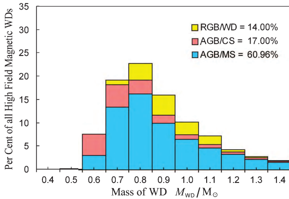
Fig. 4 Theoretical mass distribution of magnetic white dwarfs for \alpha = 0.1 . The contributions are separated according to their pre-CE progenitors. AGB= Asymptotic Giant Branch; MS= Main Sequence; RGB= Red Giant Branch; CS= Convective Star and WD=White Dwarf. Other paths also contribute but are less important than those shown. The Galactic disc age is chosen to be 9.5 Gyr
