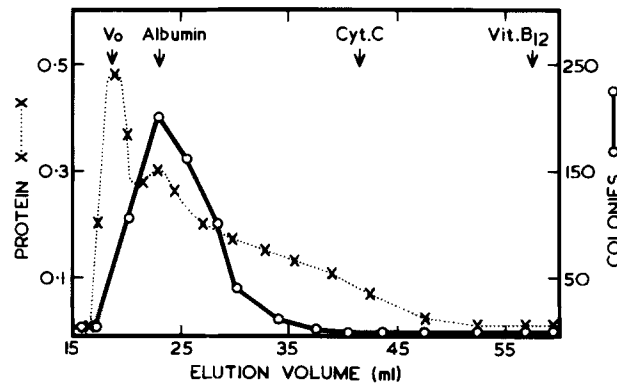
FIGURE 3 Sephadex G100 gel filtration chromatography of M-CSF eluted from DEAE-Sephacrose. The protein profile was determined by optical density at 280 nm using a 1-cm cell. The colony-stimulating activity (O—O) was measured using 0.1 ml from each fraction in the standard semisolid agar system.
