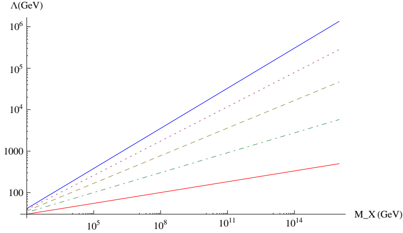
FIG. 3. Confinement scale dependence on fermion masses, in simple SUSY case, almost identical to non-SUSY, but with the confinement scale axis multiplied by \sim 10 .
