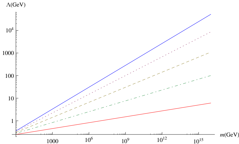
FIG. 1. Confinement scale dependence on fermion masses with five heavy and one light quark at the top through five light and one heavy quark at the bottom line. All heavy quarks have mass m and all light quarks are taken to have masses below \Lambda .
