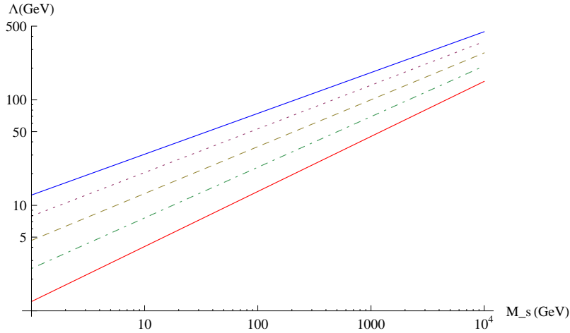
FIG. 6. As for Fig. 4 but with a dark-quark mass scale of 10^4 GeV.
