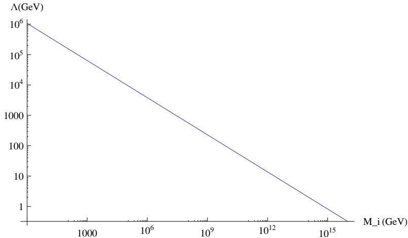
FIG. 2. The value of the confinement scale for different intermediate breaking scales M_i for the SO(10) \times SO(10) scenario of Eqs. 27-29.
