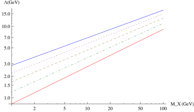
FIG. 4. Confinement scale dependence on SUSY breaking scale for fixed dark-quark mass scale of 100 GeV. The number of heavy quarks at the dark-quark mass scale ranges from five at the top to one at the bottom.
