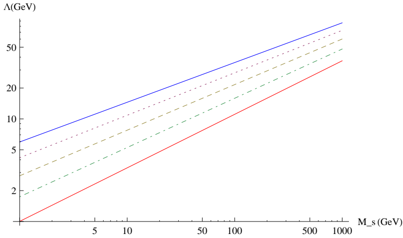
FIG. 5. As for Fig. 4 but with a dark-quark mass scale of 1000 GeV.
