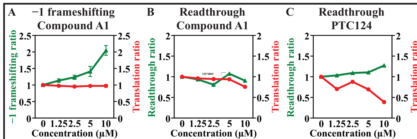
Fig 3. Frameshift enhancer A1 (A) evaluated in a dual luciferase based assay. Normalized frameshift efficiency of the HIV-1 element (green) is shown as -1 frameshift ratio relative to no compound (left ordinate). Effects of the compounds on the 0-frame control cell line containing the mutagenized slippery sequence is indicated in red, and is shown as translation ratio relative to no compound (right ordinate). (B) Compound A1 counter screen against a CFTR W1282X UGA nonsense mutant (green) and a UGG sense codon control (red). (C) PTC124 screened against CFTR W1282X (green) and the UGG sense codon control (red). Mean and standard deviation for three independent assays, each with n = 5 at 24 h.
