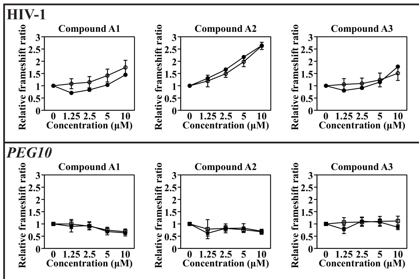
Fig 6. HIV-1 frameshift enhancers evaluated at both the HIV-1 and the PEG10 frameshift elements using dual luciferase reporters and bifluorophore reporters. Effects of enhancers A1, A2 and A3 with the bifluorophore reporters (open markers), and dual luciferase reporters (closed markers) on HIV-1 frameshifting (upper panel) and PEG10 frameshifting (lower panel) in a transient cell based assay. Results show the mean and standard deviation for quadruplicate replicates of three independent assays for the dual fluorophore assays, with the PEG10 element tested with two biological replicates in the dual luciferase assay.
