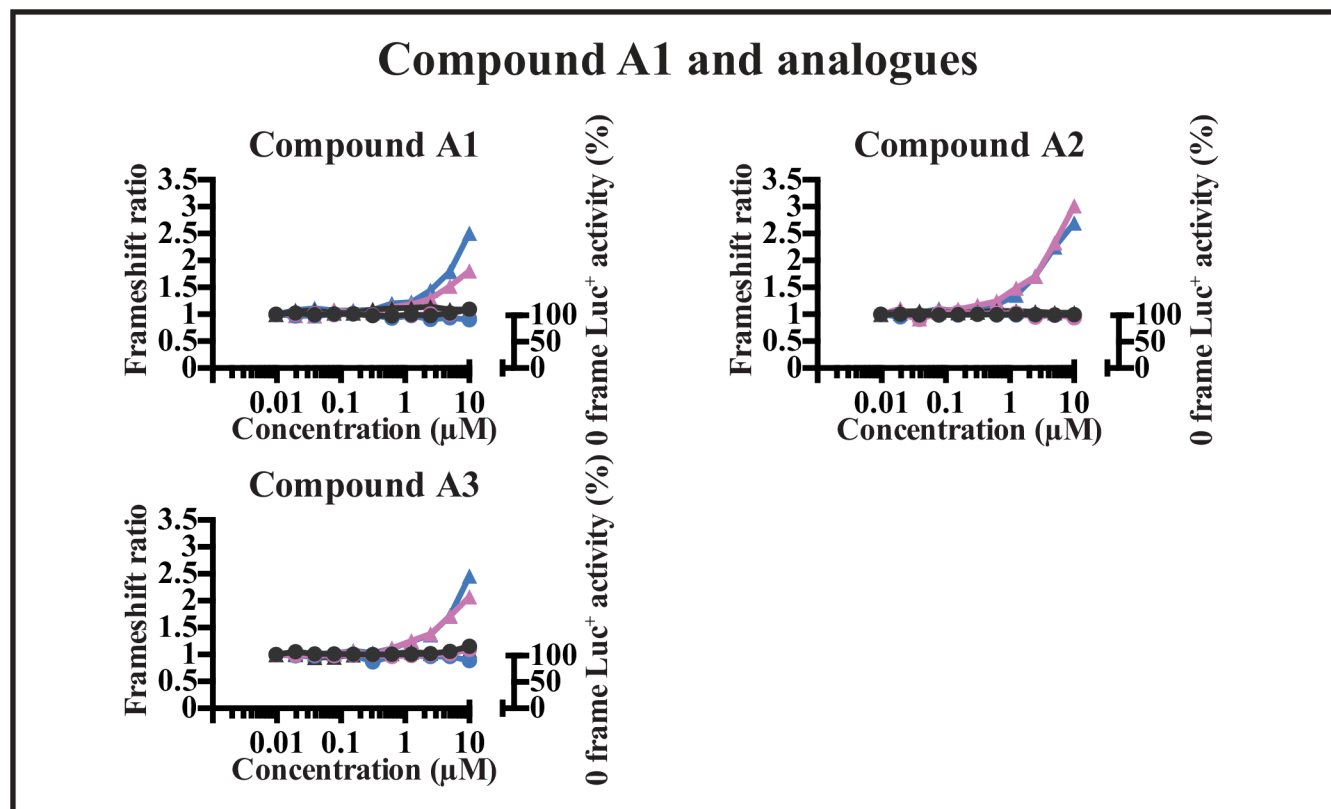
Fig 4. Effects on frameshifting at the HIV-1 element with increasing concentrations of enhancer A1 and two analogues A2 and A3 at three translational time points. The frameshift ratio of the cell line containing the HIV-1 frameshift element is indicated by triangles, as a comparison of that with no compound added. The firefly Luc + activity in the control 0-frame cell-line is indicated by circles, and is expressed as the percentage of the activity with no compound. 0 h is indicated in black, 8 h in purple and 24 h in blue.
