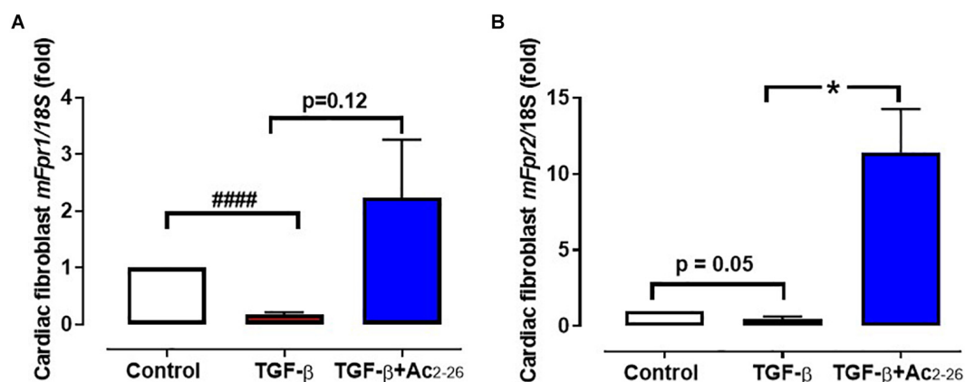
FIGURE 3 | Effect of Ac 2-26 on TGF- \beta stimulation of cardiofibroblasts in vitro . TGF- \beta (10 \mu M) downregulates ( A ) mFpr1 and ( B ) mFpr2 expression, which is elevated by Ac 2-26 (10 \mu M) within 48 h. #### P < 0.001 versus control, * P < 0.05 versus TGF- \beta -treated cells from the same cardiofibroblast preparation. One-way ANOVA with Dunnett's post-hoc test. n (number of different cardiofibroblasts preparations) = 7. Data were presented as mean \pm SEM.
