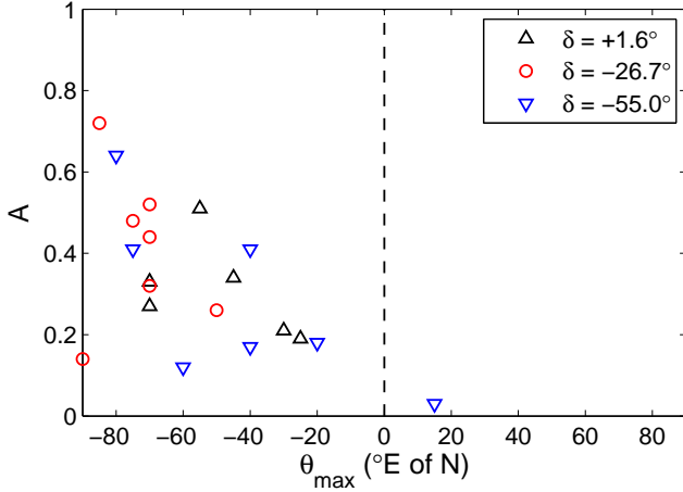
Figure 7. The degree of anisotropy of the position offset vectors, plotted against the direction of greatest position scatter, for each of the 20 datasets. Different symbols have been used to distinguish the different declination bands. The vertical dashed line separates the NW-SE quadrants ( -90^\circ to 0^\circ ) from the NE-SW quadrants ( 0^\circ to 90^\circ ).
