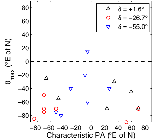
Figure 9. The direction of greatest angular position scatter, plotted against the characteristic position angle of Gaussian fits to sources in the dataset, for each of the 20 datasets. Different symbols have been used to distinguish the three declination bands. Recall that \delta = -26.7^\circ corresponds to a zenith pointing, while \delta = +1.6^\circ, -55.0^\circ are pointings \sim 30^\circ off zenith towards the north and south. A horizontal line has been drawn at 90^\circ separating the NW-SE quadrants ( -90^\circ to 0^\circ ) from the NE-SW quadrants ( 0^\circ to 90^\circ ).
