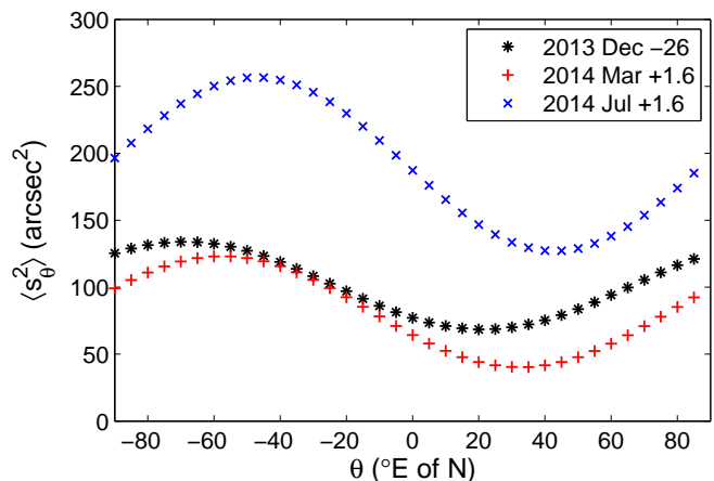
Figure 6. Position fluctuation power (squared projected offset) as a function of the angle of projection \theta , measured east of north, for the three datasets shown in Fig. 5. The power has been normalised to the number of data points (number of occurrences of any source in any snapshot) in the respective dataset.
