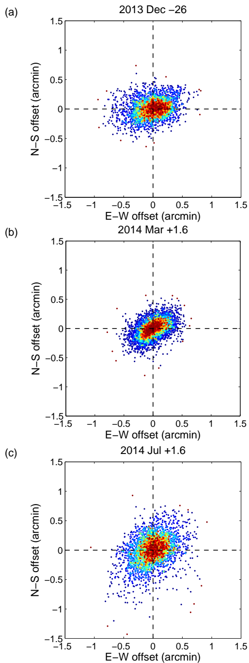
Figure 5. Position offsets for sources in the (a) 2013 Dec –26, (b) 2014 Mar +1.6 and (c) 2014 Jul +1.6 datasets, measured with respect to the time-averaged position of the source. The x axis points west and the y axis points north. The dotted lines mark the location of the origin. Points are coloured according to the local density on the page to show the shape of the distribution. Only one in five points is plotted.
