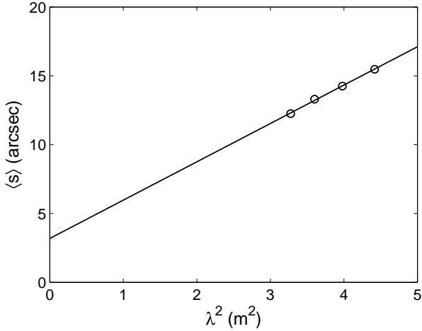
Figure 3. The magnitude of angular position offset of sources in four frequency sub-bands of the 2013 Dec –26 dataset, plotted as a function of squared wavelength. Only sources appearing in at least 20 snapshots have been included in the analysis. The line is a linear fit to the four points. The error bars on each data point associated with random fitting errors are smaller than the marker size.
