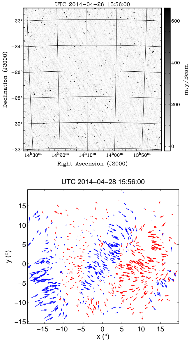
Figure 1. Top panel: An example 2-min snapshot image from 2014 Apr –26, zoomed in to the central quarter so that individual sources are visible. The full image contains of order 10^3 sources above 5\sigma . Bottom panel: The vector field of angular displacements for that snapshot, shown over the whole FoV for sources appearing in at least 20 snapshots. The middle of each arrow marks the location of a point source, and the arrow represents the displacement from its time-averaged position, with arrow lengths scaled to 150 times the actual displacement distance. The x -axis points west, the y -axis points north, and (0, 0) marks the location of the zenith (a Sanson-Flamsteed projection scheme has been used; for details, see Loi et al. 2015a). Blue and red denote arrows with positive and negative x -components, respectively, to aid visualisation. Organised patches of motion are clearly evident, corresponding to density structures with length scales of \sim 50 km for an assumed altitude of 300 km.
