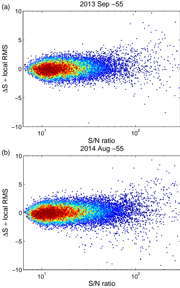
Figure 8. Scatter plots of the difference between measured and mean flux density \Delta S versus the mean flux density S (each axis normalised by the local RMS), for (a) 2013 Sep –55 and (b) 2014 Aug –55, the two datasets with the lowest and highest average amplitude of position fluctuations, respectively. The horizontal axis is shown on a logarithmic scale. Points are coloured by the local density on the page to show the shape of the distribution. Only one in five points is plotted. Note that the taper (drop in source counts) for S/N ratios below 10, despite faint sources being much more common than bright sources, is due to a sample selection effect: we required that sources appear in a large number of snapshots, biasing our sample to exclude fainter sources that might be lost in regions of high image RMS.
