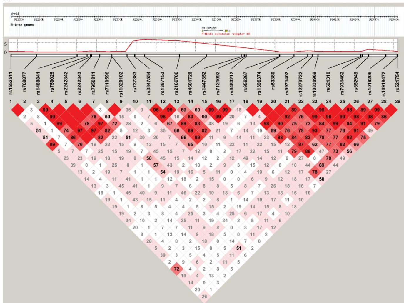
FIG. 1. Genomic context of melatonin receptor MTNR1B region showing pairwise LD between SNPs with minor allele frequency \geq 0.05 directly genotyped in both Indian Asians (A) and European Caucasians (B) using Haploview's standard color scheme.
