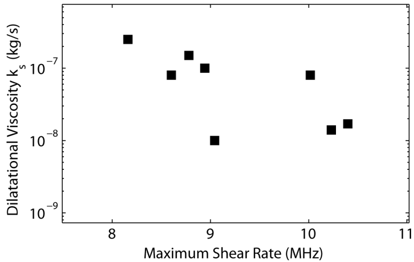
Figure 4. The relationship between the shell dilatational viscosity and maximum shear rate.
