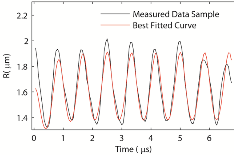
Figure 1. A sample best-fit data for LSMBs using Marmottant’s model. The bubble was driven at 1.2 MHz and an acoustic pressure of 290 kPa. The best-fit shell parameters are \chi = 0.12 N/m and \kappa_s = 9.0 \times 10^{-8} kg/s, with R_0 = 1.63 \mu\text{m} .
