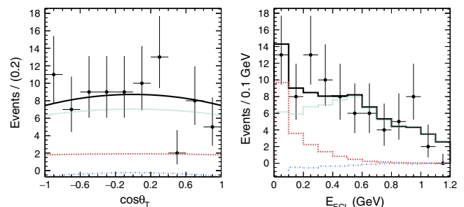
FIG. 5. Projections of the fit result on \cos \theta_T (left) and E_{\text{ECL}} (right) for B^0 \rightarrow \text{invisible} . Dots with error bars are data, black solid line is the fit result, red dotted line is the signal component, green short-dashed line is the generic B background component and blue dash-dotted line is the non- B background component.
