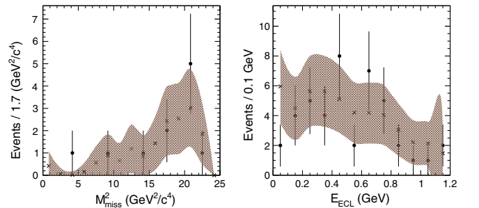
FIG. 7. M_{\text{miss}}^2 (left) and E_{\text{ECL}} (right) distributions of data and the expected background for B^0 \rightarrow invisible + \gamma . The M_{\text{miss}}^2 distribution is plotted in the E_{\text{ECL}} signal box and the E_{\text{ECL}} distribution is plotted in the whole M_{\text{miss}}^2 region. The black points with error are data. The gray crosses with a shaded error band are the expected background.
