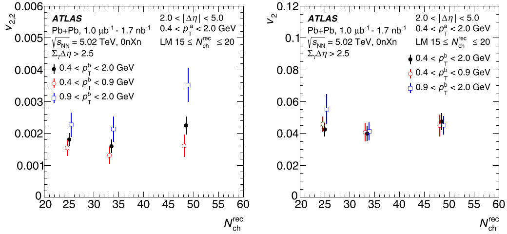
FIG. 13. Summary of the factorization test for v_2 values as a function of N_{\text{ch}}^{\text{rec}} . Comparison of v_{2,2} values (left) and derived v_2 values (right) using the same particle a selection, but different selections on particle b . Only statistical uncertainties are shown. The points are displaced horizontally for visibility.
