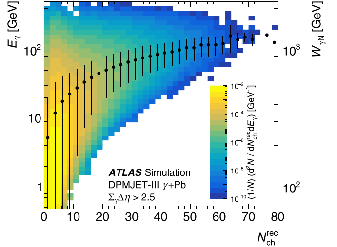
FIG. 6. Correlation between photon energy E_\gamma and event multiplicity N_{\text{ch}}^{\text{rec}} in simulated DPMJET-III \gamma + \text{Pb} events. The right-hand axis shows the center-of-mass energy W for the photon-nucleon collision system. The markers and vertical error bars show the mean and standard deviation, respectively, of E_\gamma as a function of N_{\text{ch}}^{\text{rec}} .
