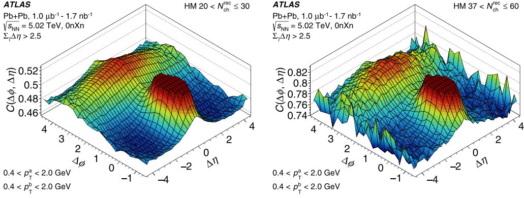
FIG. 7. Two-dimensional normalized particle pair distributions in photonuclear events, corrected for acceptance effects with the mixed-event distribution, and presented as a function of \Delta\eta and \Delta\phi . The peak at (\Delta\phi, \Delta\eta) = (0, 0) is truncated to better show the structure of the correlation function. Each panel represents a different charged-particle multiplicity N_{\text{ch}}^{\text{rec}} range for the selection 0.4 < (p_{\text{T}}^a, p_{\text{T}}^b) < 2.0 GeV.
