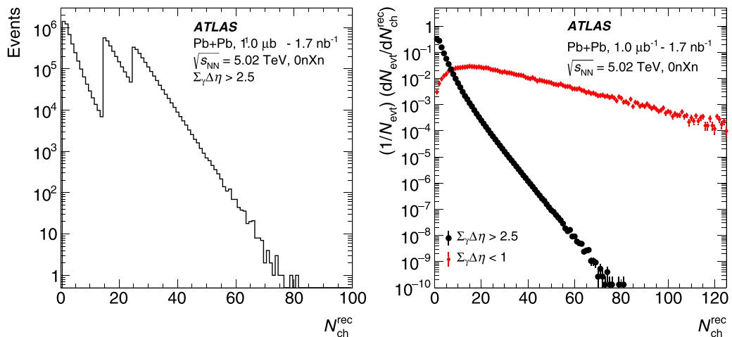
FIG. 3. Left: Distribution of event charged-particle multiplicity, N_{\text{ch}}^{\text{rec}} , for the photonuclear event selection from multiple triggers, without prescale correction. Right: Distribution of event charged-particle multiplicity, N_{\text{ch}}^{\text{rec}} , for the photonuclear event selection (black) with corrections for trigger efficiency and prescale factors, and an alternative selection intended to select hadronic Pb+Pb events (red, see text).
