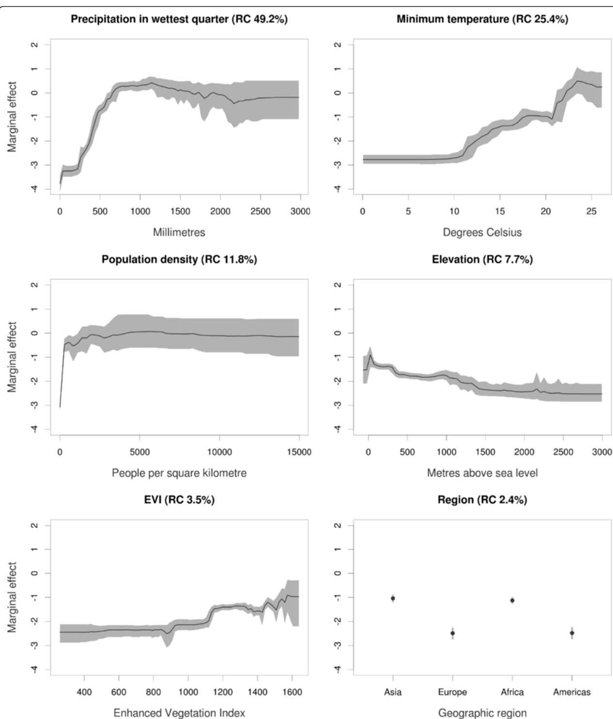
Figure 4 Marginal effect curves for each covariate used in the ensemble of 120 boosted regression tree (BRT) models. Black lines represent the mean marginal effect over all 120 BRT ensembles and grey envelopes the 95% bootstrap confidence interval. The y-axis is the untransformed logit response and x-axis is the full range of covariates values. The percentage values in parenthesis show the mean relative contribution of the covariate over all 120 sub-models of the ensemble.
