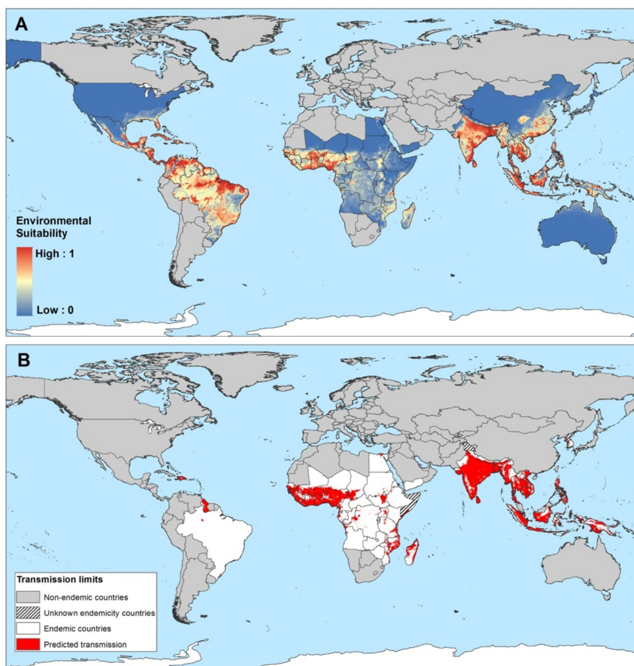
Figure 5 Global environmental suitability (A) and limits (B) of lymphatic filariasis transmission as predicted by the final boosted regression trees model. Countries that have never reported LF endemic infections are masked in grey, and areas suitable for LF transmission, as predicted by the BRT model, are displayed in red (B).
