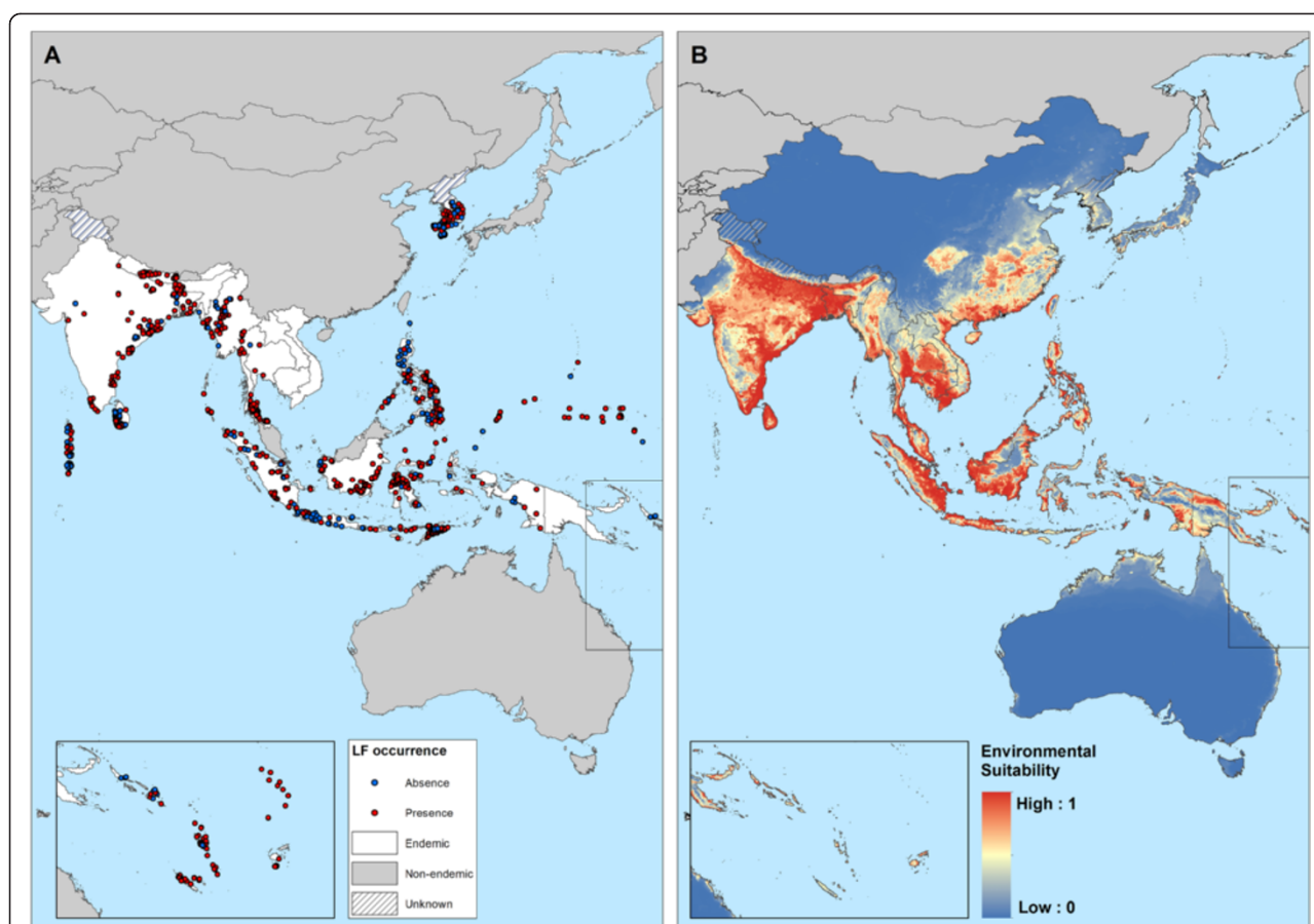
Figure 9 Reported and predicted distribution of lymphatic filariasis in South-Asia and Western Pacific. (A) Observed occurrence and absence of LF and (B) environmental suitability for lymphatic filariasis transmission, as predicted by the final boosted regression trees model, in South-east Asia and western Pacific.
