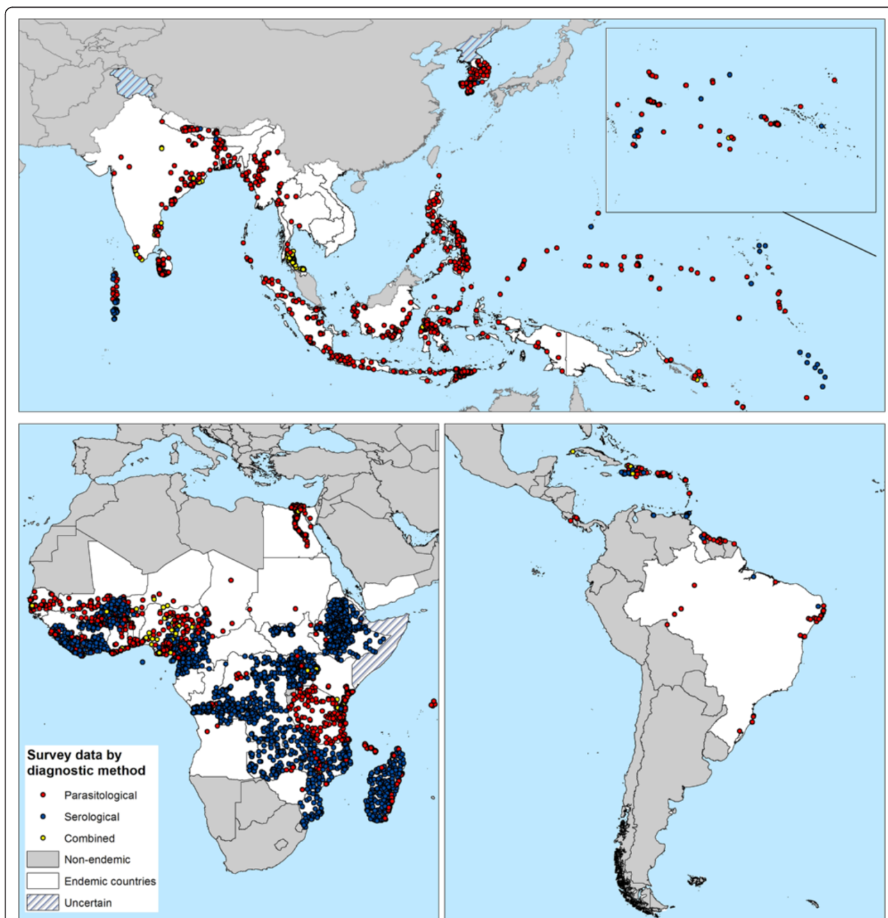
Figure 3 The global distribution of data points included in the Global Atlas Lymphatic Filariasis database by diagnostic method. Red = parasitological methods; blue = serological methods; and yellow = combination of methods.
