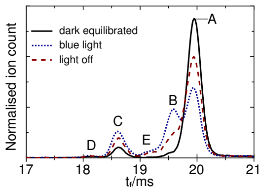
Fig. 3 ATDs for RPSB for different pre-treatments of the electrosprayed solution. Dark equilibrated: RPSB solution in dark at -20^{\circ}\text{C} for 2 hours prior to electrospray ionization. Blue light: RPSB solution exposed to 460 nm light for 1 hr. Light off: 2 hrs after 460 nm light was blocked. The RF drive voltage to IF1 was switched off, to avoid collision induced isomerization.
