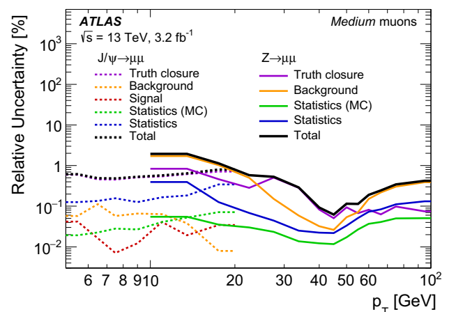
Fig. 2 Total uncertainty in the efficiency scale factor for Medium muons as a function of p_T as obtained from Z \rightarrow \mu\mu (solid lines) and J/\psi \rightarrow \mu\mu (dashed lines) decays. The combined uncertainty is the sum in quadrature of the individual contributions
