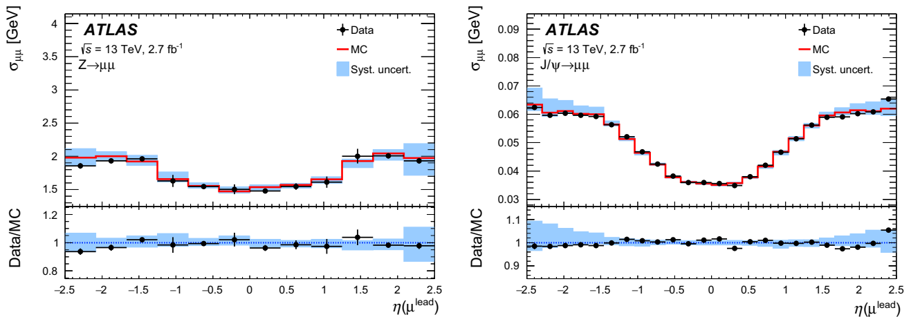
Fig. 11 Dimuon invariant mass resolution for CB muons for Z \rightarrow \mu\mu (left) and J/\psi \rightarrow \mu\mu (right) events for data and corrected simulation as a function of the pseudorapidity of the highest- p_T muon. The upper panels show the fitted resolution value for data and corrected simulation.
