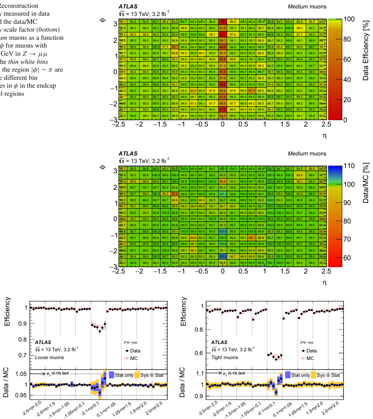
Fig. 5 Muon reconstruction efficiency in different \eta regions measured in J/\psi \rightarrow \mu\mu events for Loose (left) and Tight (right) muon selections. Within each \eta region, the efficiency is measured in six p_T bins (5–6, 6–7, 7–8, 8–10, 10–12, and 12–15 GeV). The resulting values are plotted as distinct measurements in each \eta bin with p_T increasing from 5 to
