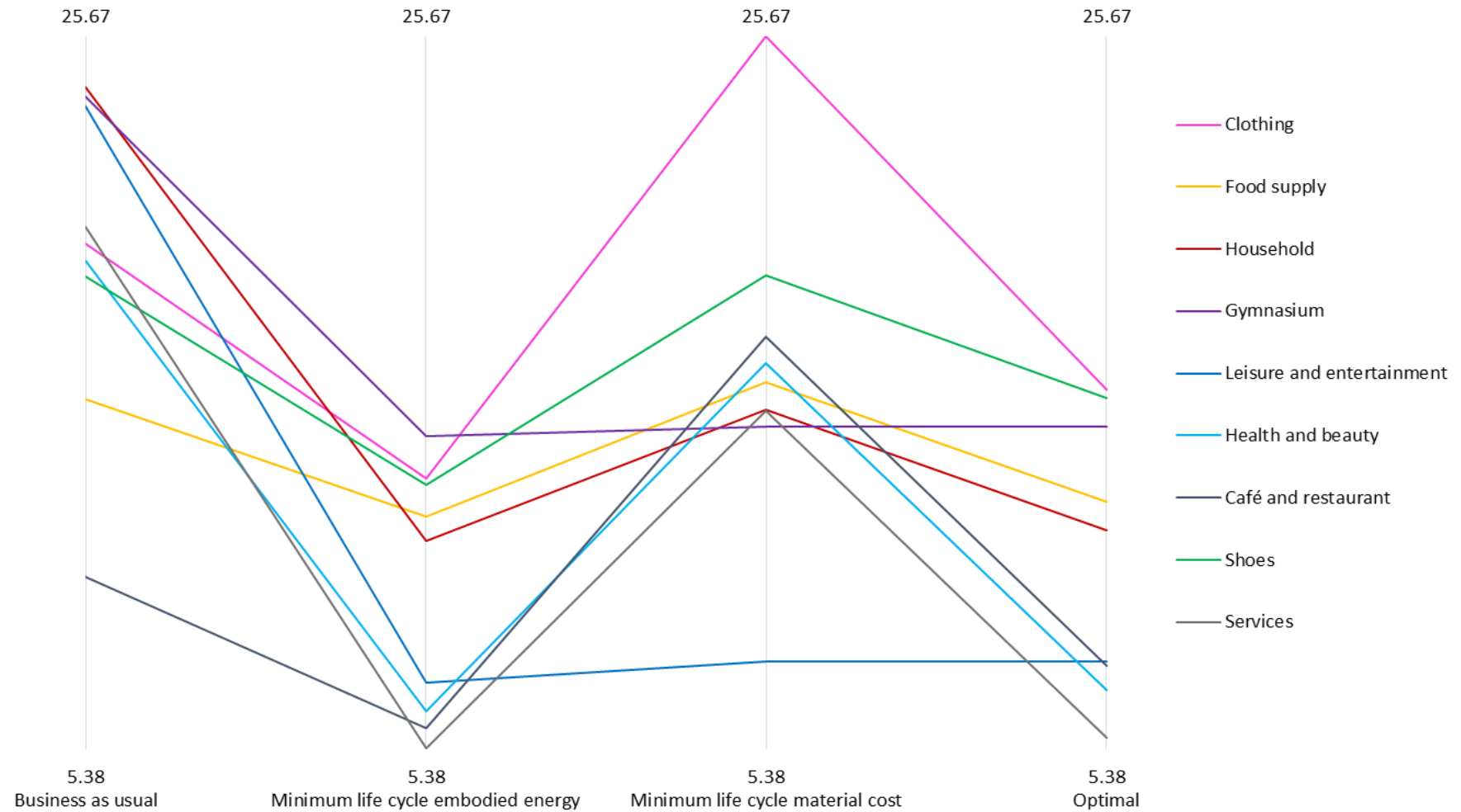
Figure 7.19: Comparison of life cycle embodied energy per unit area (in GJ/m²) of different specialty shop types in shopping centres
