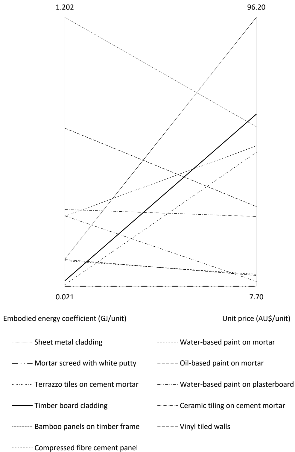
Figure 7.3 C: Parallel coordinates graph of embodied energy coefficients and unit prices of wall finishes assemblies
